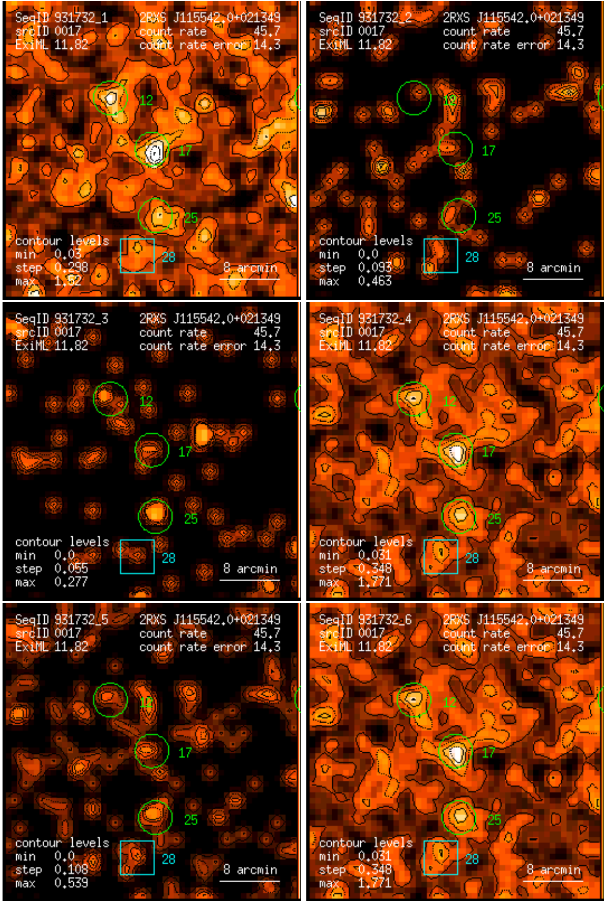
Figure 17: RASS 931732: detection 0017: band rate images, Gaussian filter: (1) PSPC channels 11 – 41, (2) 52 – 90, (3) 91 – 201, (4) 11 – 235, (5) 52 – 201, (6) 11 – 201. Broad band rates in counts/ks. Band rate contour levels in counts/ks/arcmin 2 .
