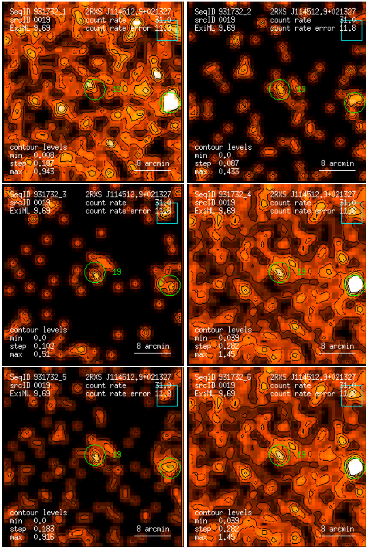
Figure 19: RASS 931732: detection 0019: band rate images, Gaussian filter: (1) PSPC channels 11 – 41, (2) 52 – 90, (3) 91 – 201, (4) 11 – 235, (5) 52 – 201, (6) 11 – 201. Broad band rates in counts/ks. Band rate contour levels in counts/ks/arcmin 2 .
