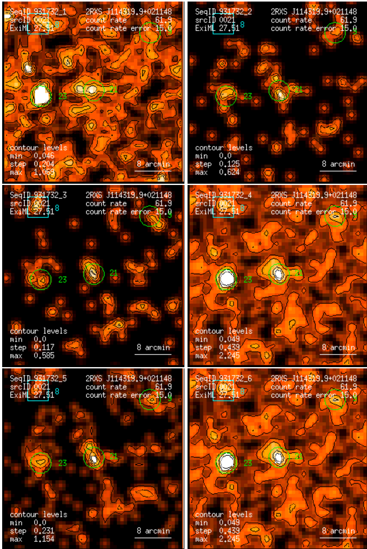
Figure 21: RASS 931732: detection 0021: band rate images, Gaussian filter: (1) PSPC channels 11 – 41, (2) 52 – 90, (3) 91 – 201, (4) 11 – 235, (5) 52 – 201, (6) 11 – 201. Broad band rates in counts/ks. Band rate contour levels in counts/ks/arcmin 2 .
