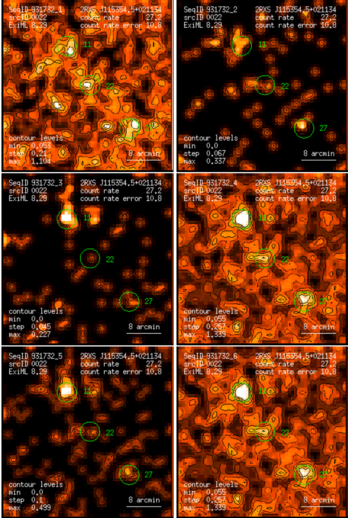
Figure 22: RASS 931732: detection 0022: band rate images, Gaussian filter: (1) PSPC channels 11 – 41, (2) 52 – 90, (3) 91 – 201, (4) 11 – 235, (5) 52 – 201, (6) 11 – 201. Broad band rates in counts/ks. Band rate contour levels in counts/ks/arcmin 2 .
