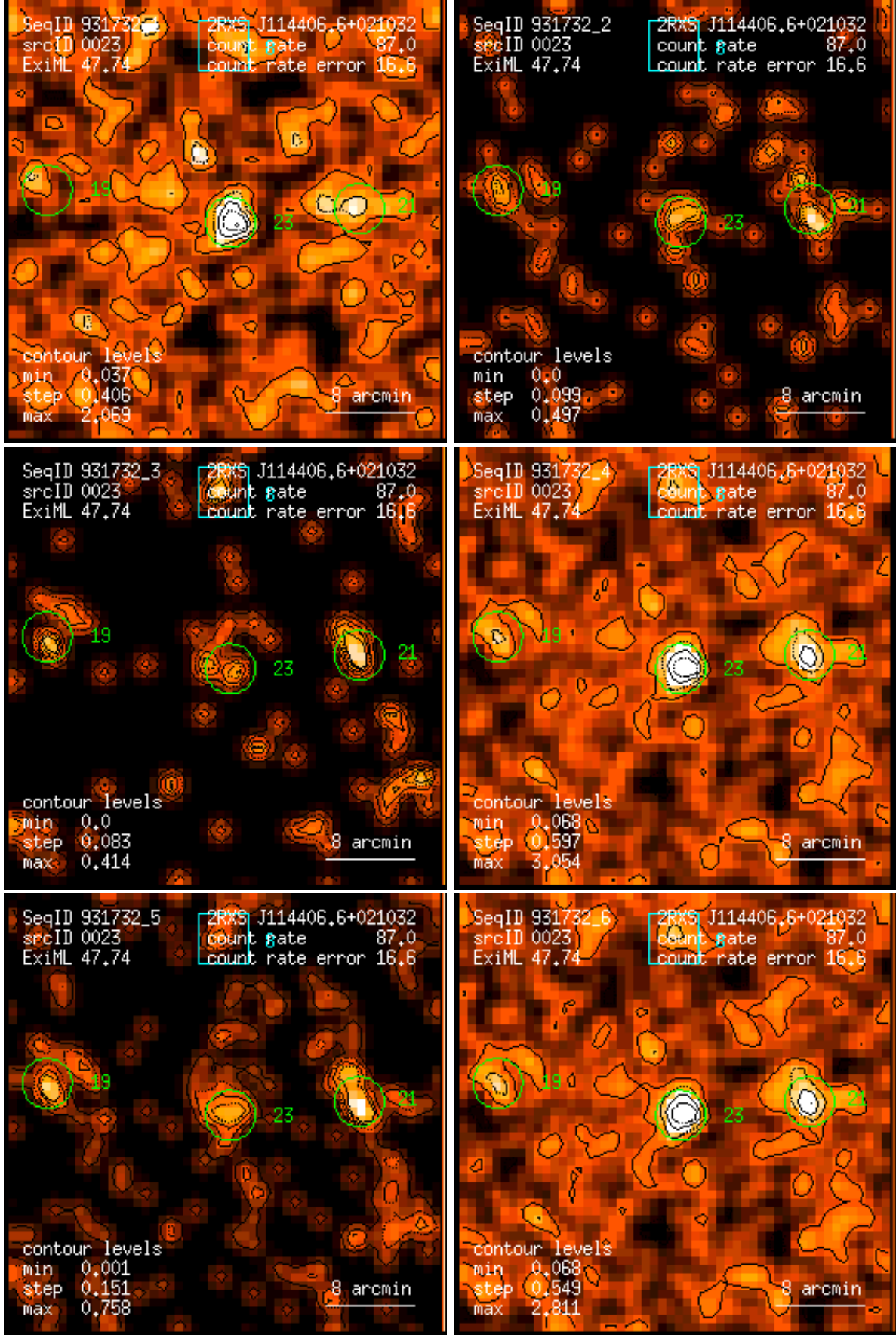
Figure 23: RASS 931732: detection 0023: band rate images, Gaussian filter: (1) PSPC channels 11 – 41, (2) 52 – 90, (3) 91 – 201, (4) 11 – 235, (5) 52 – 201, (6) 11 – 201. Broad band rates in counts/ks. Band rate contour levels in counts/ks/arcmin 2 .
