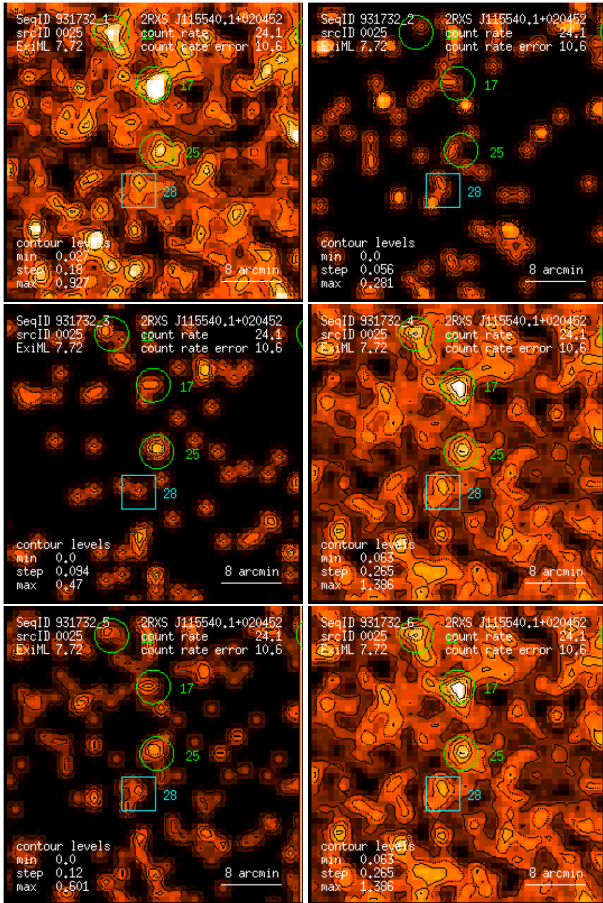
Figure 25: RASS 931732: detection 0025: band rate images, Gaussian filter: (1) PSPC channels 11 – 41, (2) 52 – 90, (3) 91 – 201, (4) 11 – 235, (5) 52 – 201, (6) 11 – 201. Broad band rates in counts/ks. Band rate contour levels in counts/ks/arcmin 2 .
