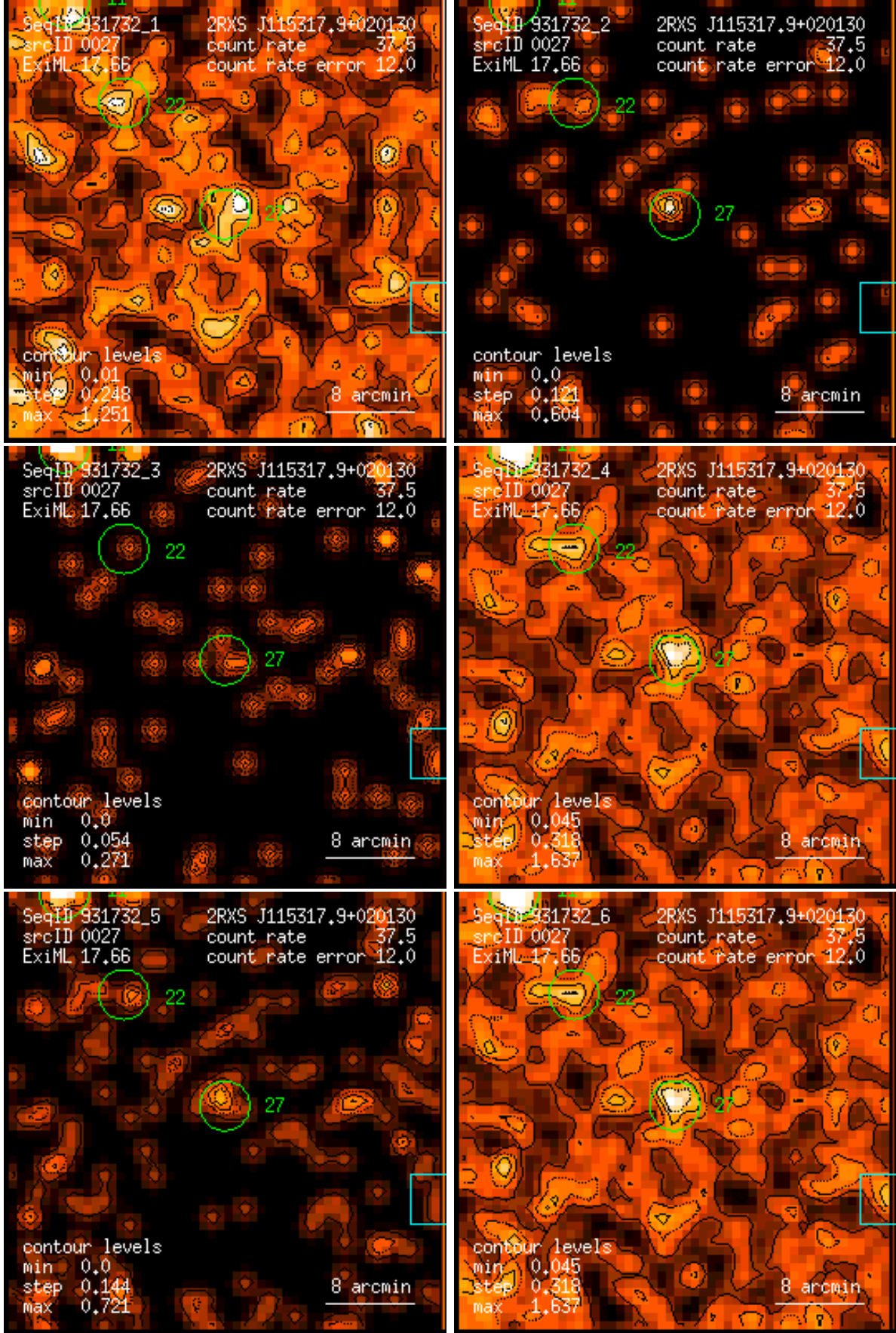
Figure 27: RASS 931732: detection 0027: band rate images, Gaussian filter: (1) PSPC channels 11 – 41, (2) 52 – 90, (3) 91 – 201, (4) 11 – 235, (5) 52 – 201, (6) 11 – 201. Broad band rates in counts/ks. Band rate contour levels in counts/ks/arcmin 2 .
