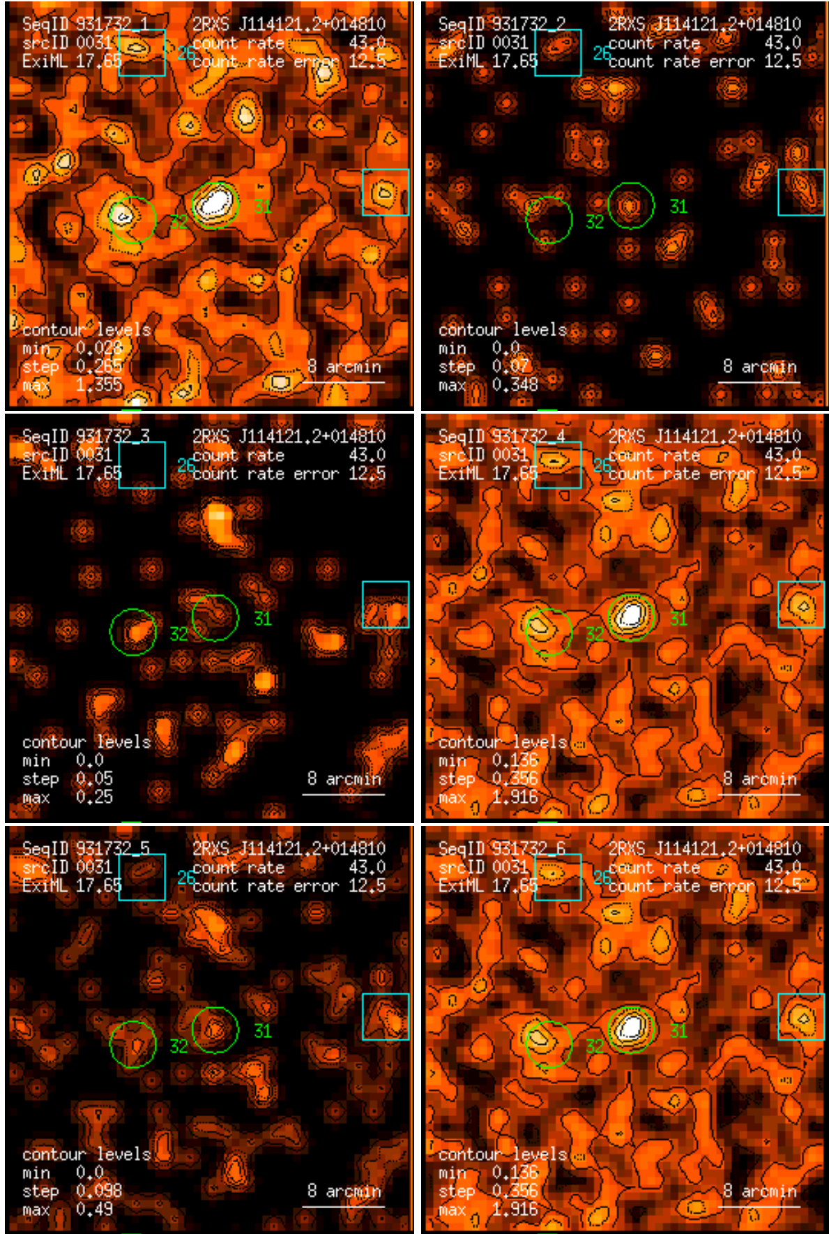
Figure 31: RASS 931732: detection 0031: band rate images, Gaussian filter: (1) PSPC channels 11 – 41, (2) 52 – 90, (3) 91 – 201, (4) 11 – 235, (5) 52 – 201, (6) 11 – 201. Broad band rates in counts/ks. Band rate contour levels in counts/ks/arcmin 2 .
