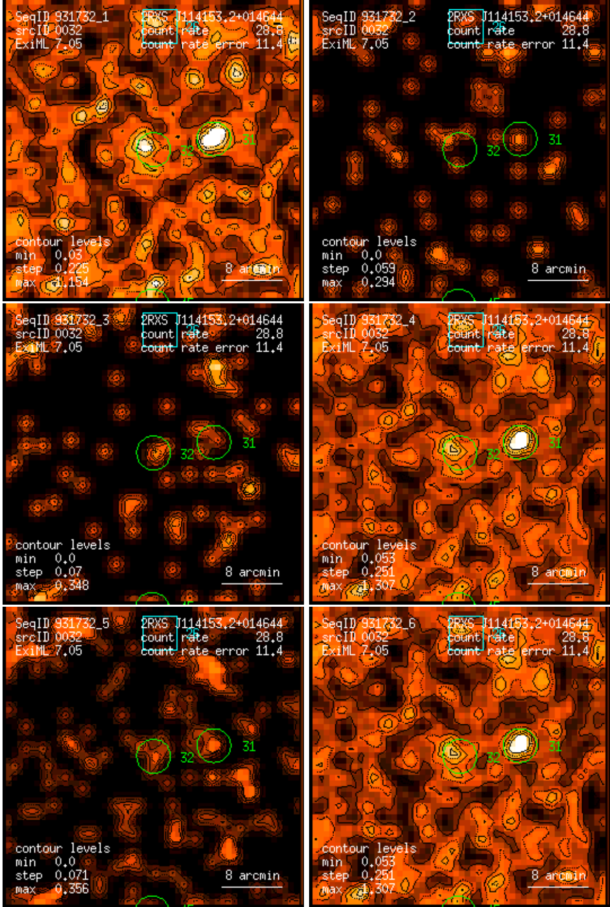
Figure 32: RASS 931732: detection 0032: band rate images, Gaussian filter: (1) PSPC channels 11 – 41, (2) 52 – 90, (3) 91 – 201, (4) 11 – 235, (5) 52 – 201, (6) 11 – 201. Broad band rates in counts/ks. Band rate contour levels in counts/ks/arcmin 2 .
