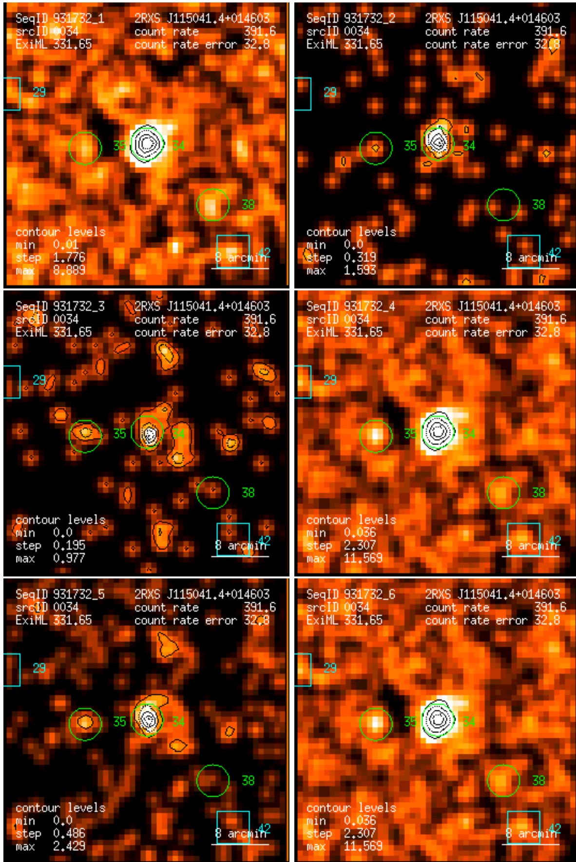
Figure 34: RASS 931732: detection 0034: band rate images, Gaussian filter: (1) PSPC channels 11 – 41, (2) 52 – 90, (3) 91 – 201, (4) 11 – 235, (5) 52 – 201, (6) 11 – 201. Broad band rates in counts/ks. Band rate contour levels in counts/ks/arcmin 2 .
