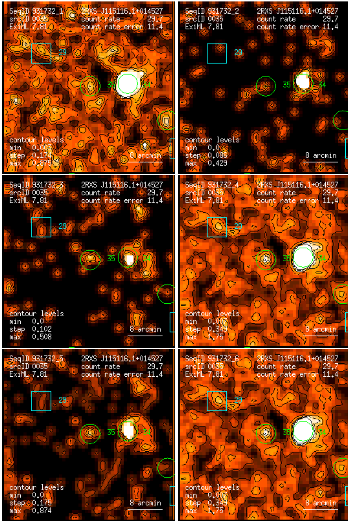
Figure 35: RASS 931732: detection 0035: band rate images, Gaussian filter: (1) PSPC channels 11 – 41, (2) 52 – 90, (3) 91 – 201, (4) 11 – 235, (5) 52 – 201, (6) 11 – 201. Broad band rates in counts/ks. Band rate contour levels in counts/ks/arcmin 2 .
