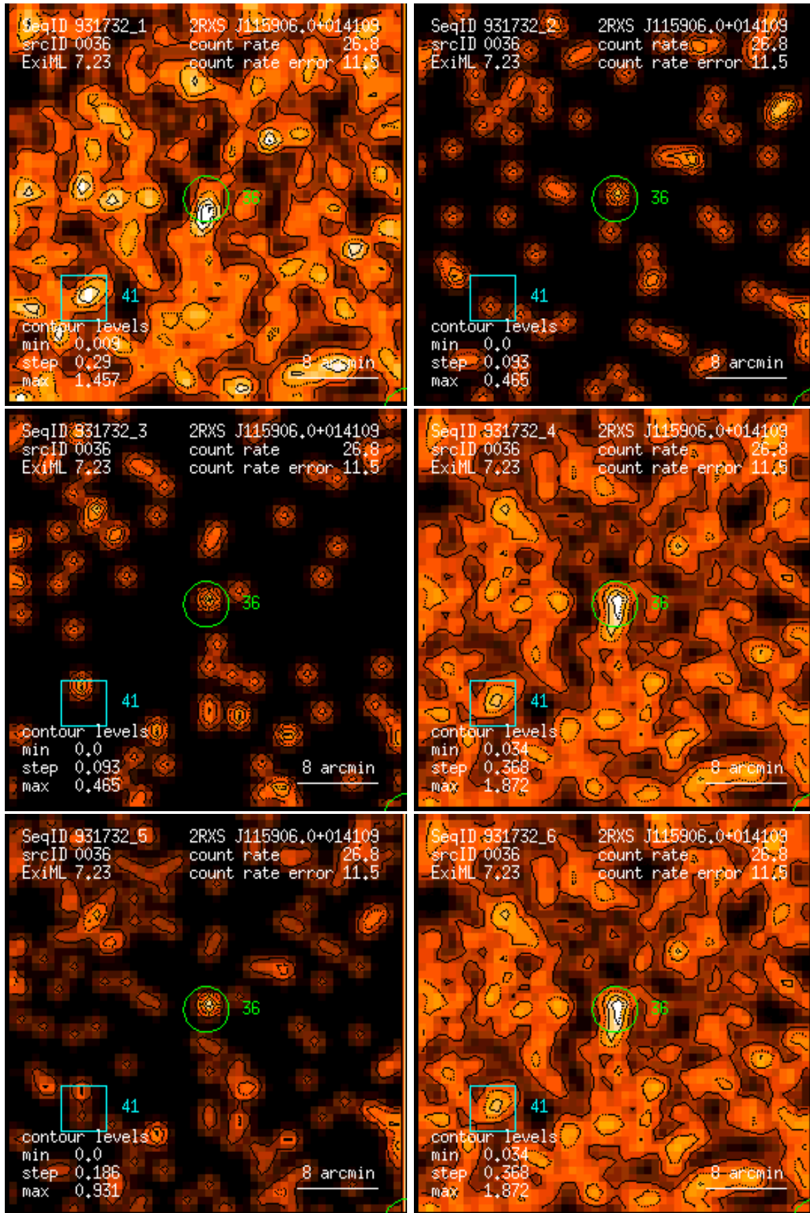
Figure 36: RASS 931732: detection 0036: band rate images, Gaussian filter: (1) PSPC channels 11 – 41, (2) 52 – 90, (3) 91 – 201, (4) 11 – 235, (5) 52 – 201, (6) 11 – 201. Broad band rates in counts/ks. Band rate contour levels in counts/ks/arcmin 2 .
