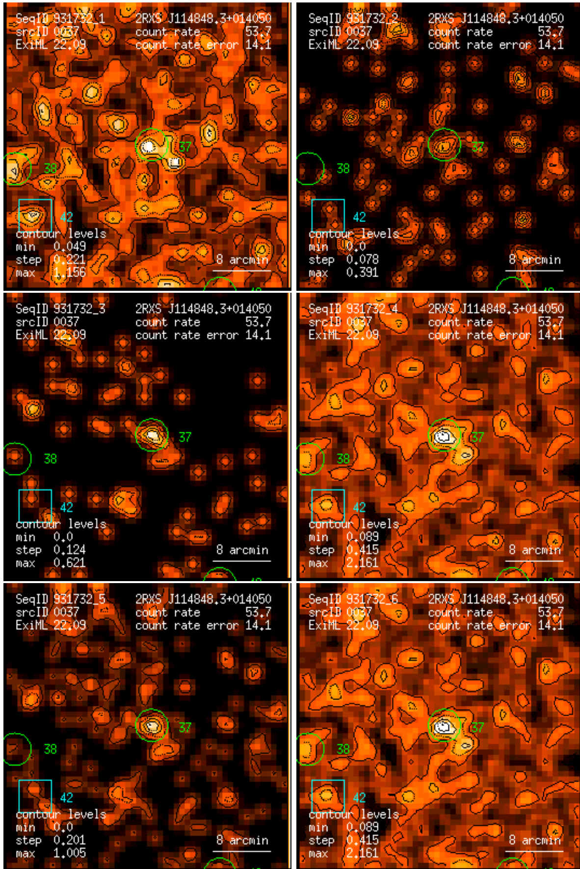
Figure 37: RASS 931732: detection 0037: band rate images, Gaussian filter: (1) PSPC channels 11 – 41, (2) 52 – 90, (3) 91 – 201, (4) 11 – 235, (5) 52 – 201, (6) 11 – 201. Broad band rates in counts/ks. Band rate contour levels in counts/ks/arcmin 2 .
