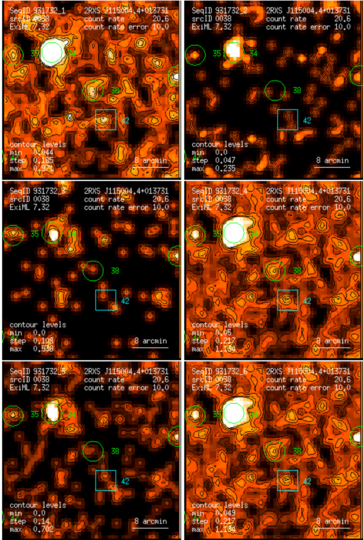
Figure 38: RASS 931732: detection 0038: band rate images, Gaussian filter: (1) PSPC channels 11 – 41, (2) 52 – 90, (3) 91 – 201, (4) 11 – 235, (5) 52 – 201, (6) 11 – 201. Broad band rates in counts/ks. Band rate contour levels in counts/ks/arcmin 2 .
