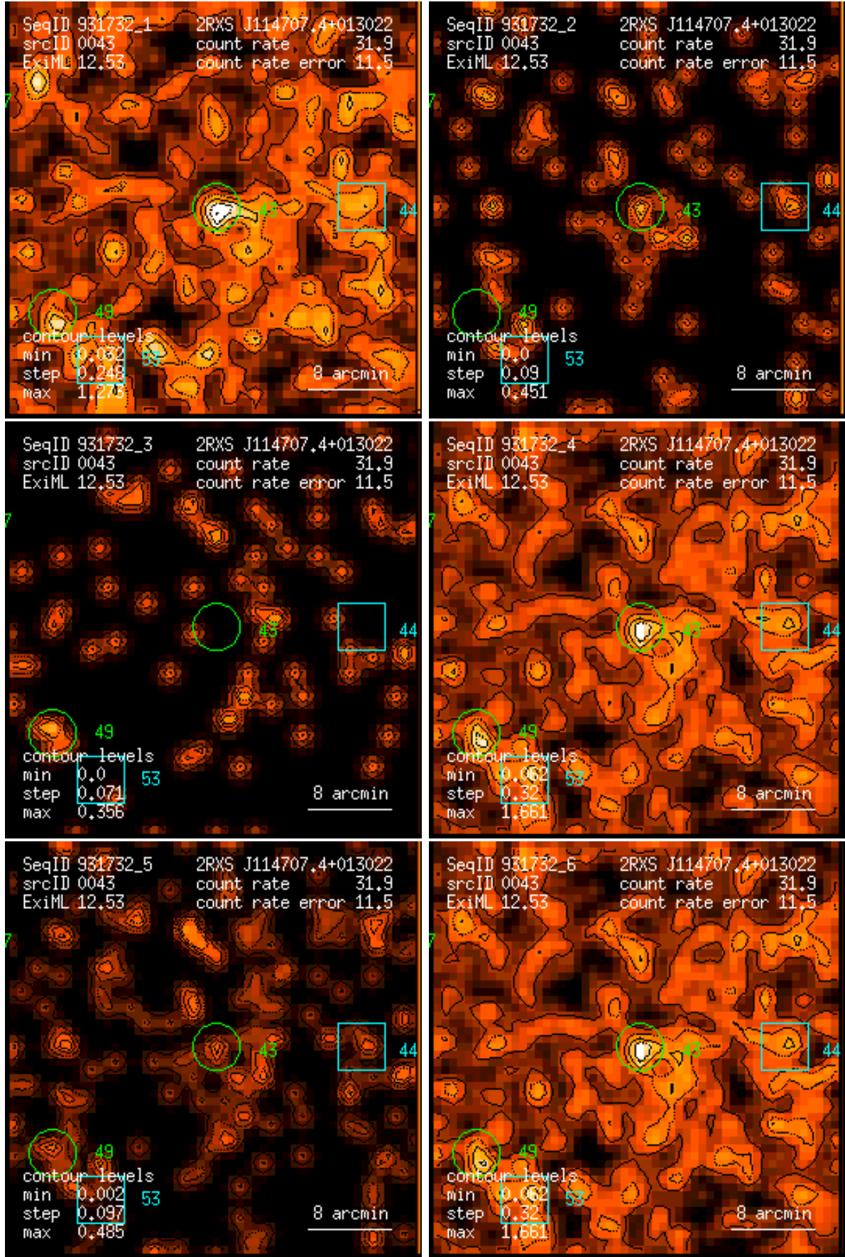
Figure 43: RASS 931732: detection 0043: band rate images, Gaussian filter: (1) PSPC channels 11 – 41, (2) 52 – 90, (3) 91 – 201, (4) 11 – 235, (5) 52 – 201, (6) 11 – 201. Broad band rates in counts/ks. Band rate contour levels in counts/ks/arcmin 2 .
