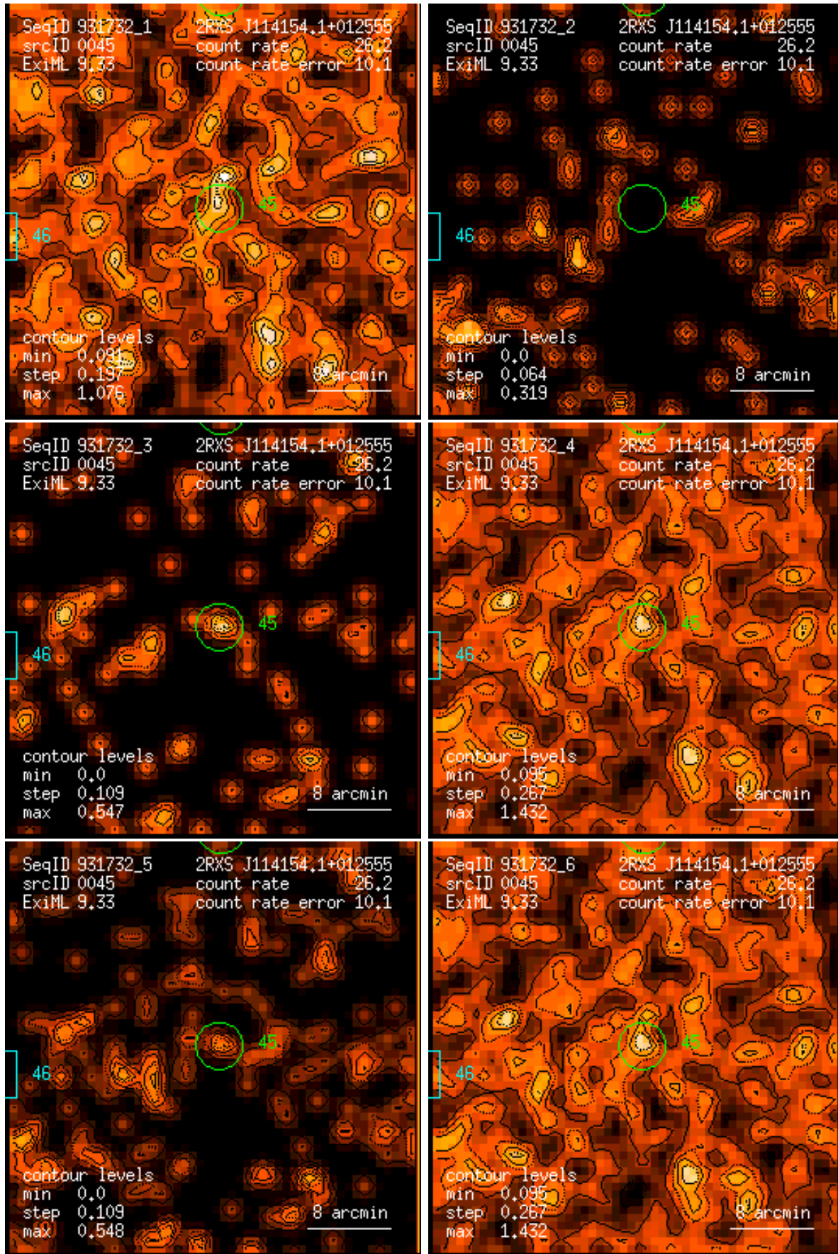
Figure 45: RASS 931732: detection 0045: band rate images, Gaussian filter: (1) PSPC channels 11 – 41, (2) 52 – 90, (3) 91 – 201, (4) 11 – 235, (5) 52 – 201, (6) 11 – 201. Broad band rates in counts/ks. Band rate contour levels in counts/ks/arcmin 2 .
