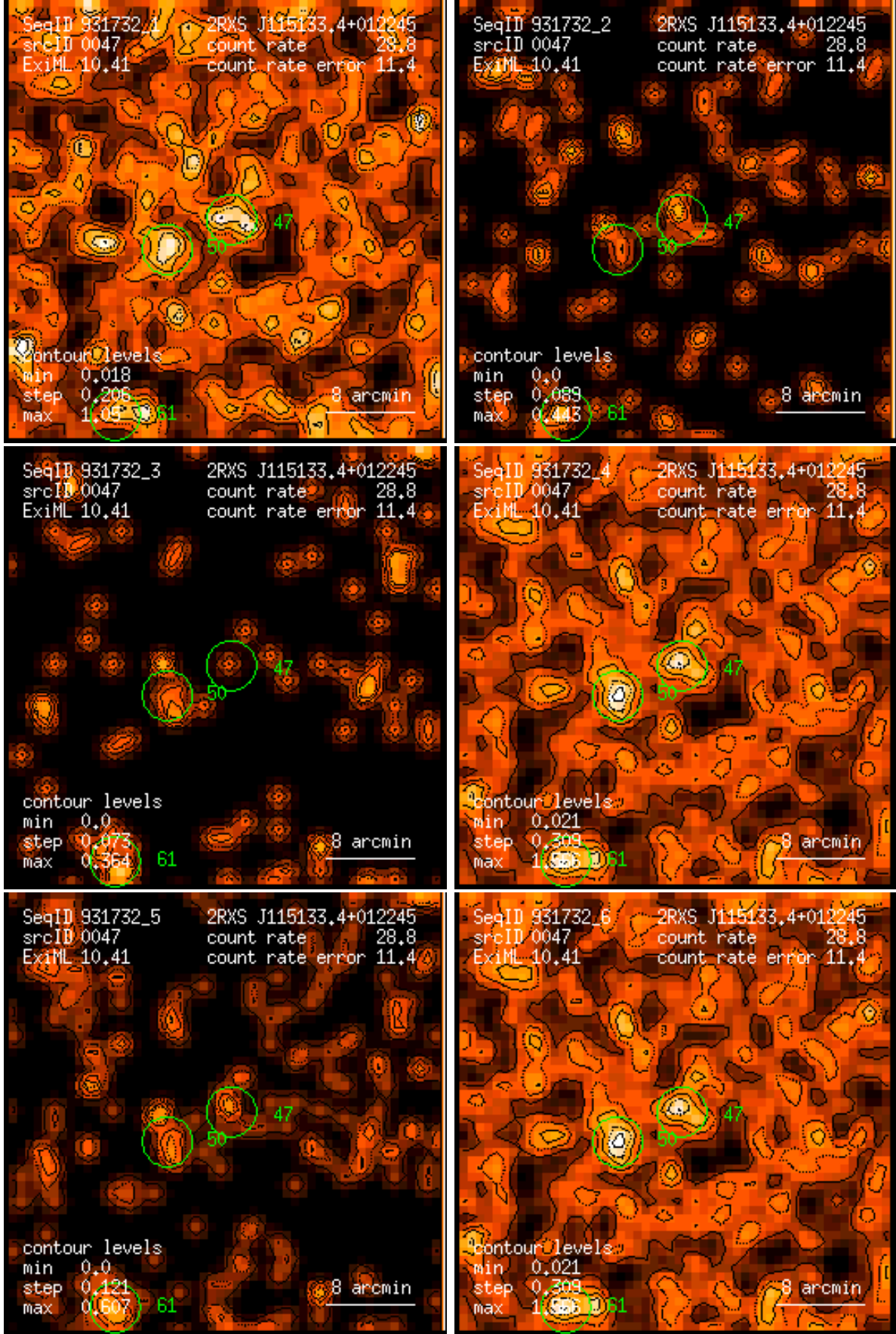
Figure 47: RASS 931732: detection 0047: band rate images, Gaussian filter: (1) PSPC channels 11 – 41, (2) 52 – 90, (3) 91 – 201, (4) 11 – 235, (5) 52 – 201, (6) 11 – 201. Broad band rates in counts/ks. Band rate contour levels in counts/ks/arcmin 2 .
