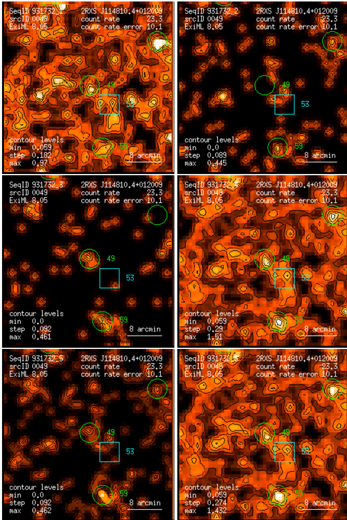
Figure 49: RASS 931732: detection 0049: band rate images, Gaussian filter: (1) PSPC channels 11 – 41, (2) 52 – 90, (3) 91 – 201, (4) 11 – 235, (5) 52 – 201, (6) 11 – 201. Broad band rates in counts/ks. Band rate contour levels in counts/ks/arcmin 2 .
