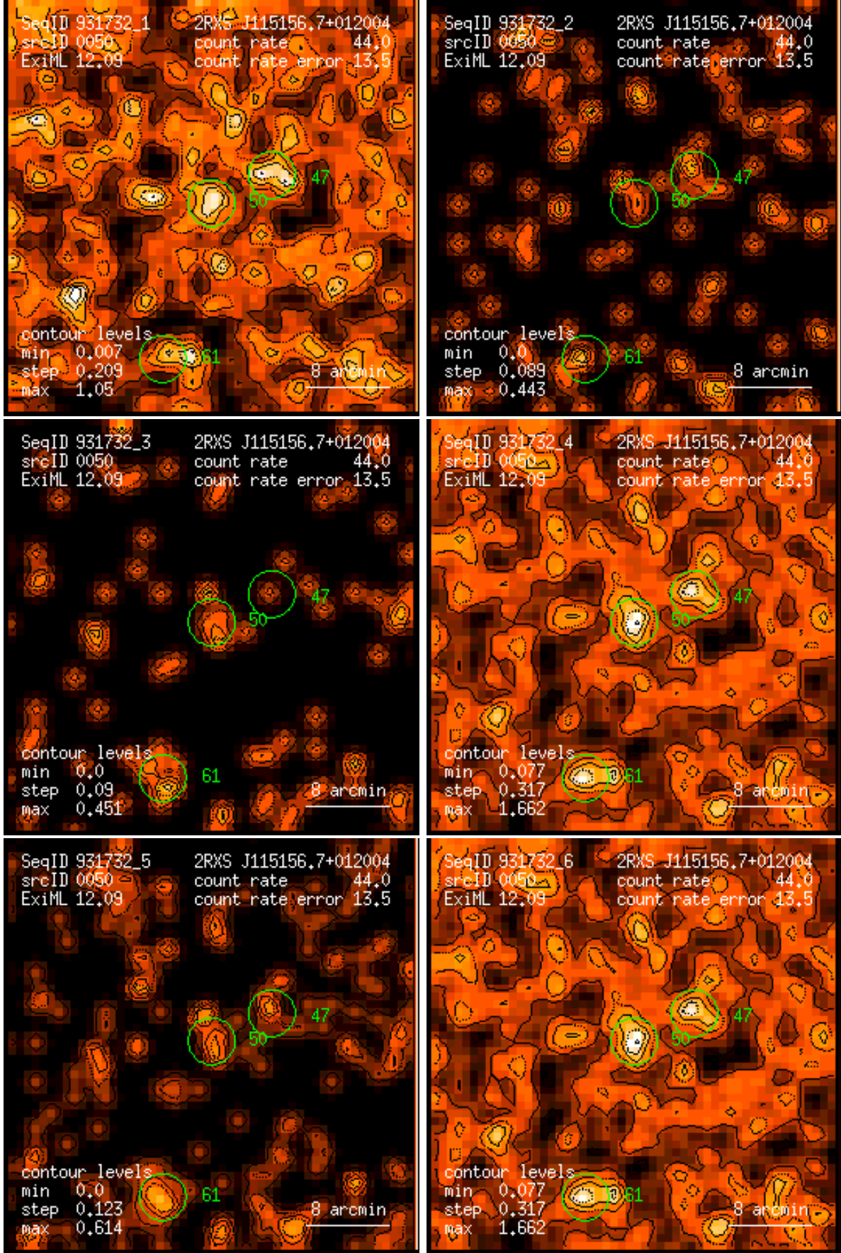
Figure 50: RASS 931732: detection 0050: band rate images, Gaussian filter: (1) PSPC channels 11 – 41, (2) 52 – 90, (3) 91 – 201, (4) 11 – 235, (5) 52 – 201, (6) 11 – 201. Broad band rates in counts/ks. Band rate contour levels in counts/ks/arcmin 2 .
