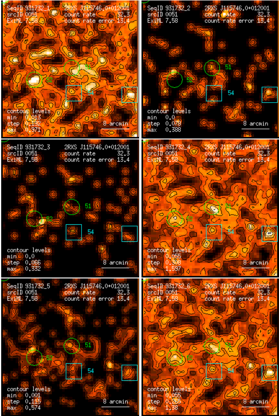
Figure 51: RASS 931732: detection 0051: band rate images, Gaussian filter: (1) PSPC channels 11 – 41, (2) 52 – 90, (3) 91 – 201, (4) 11 – 235, (5) 52 – 201, (6) 11 – 201. Broad band rates in counts/ks. Band rate contour levels in counts/ks/arcmin 2 .
