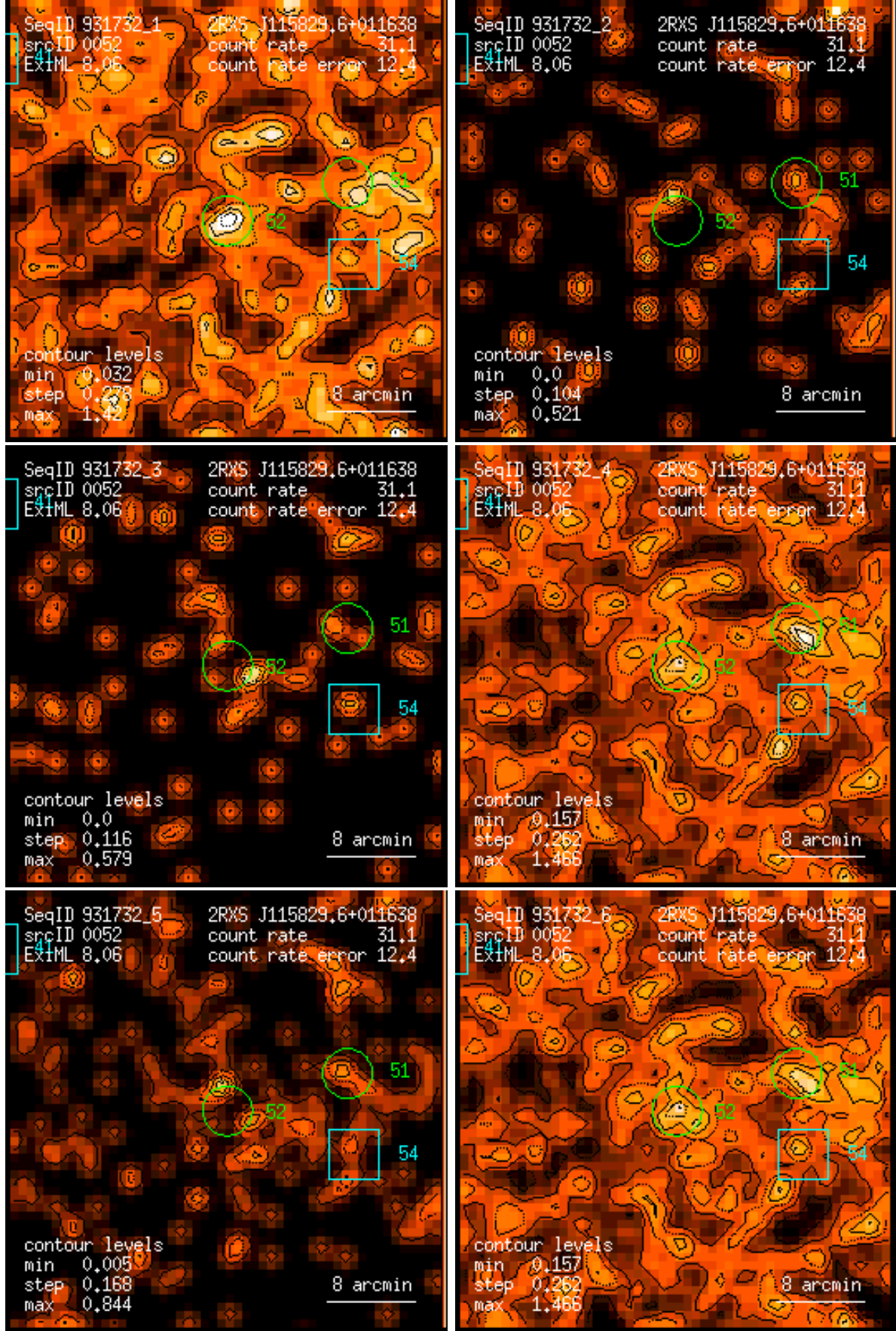
Figure 52: RASS 931732: detection 0052: band rate images, Gaussian filter: (1) PSPC channels 11 – 41, (2) 52 – 90, (3) 91 – 201, (4) 11 – 235, (5) 52 – 201, (6) 11 – 201. Broad band rates in counts/ks. Band rate contour levels in counts/ks/arcmin 2 .
