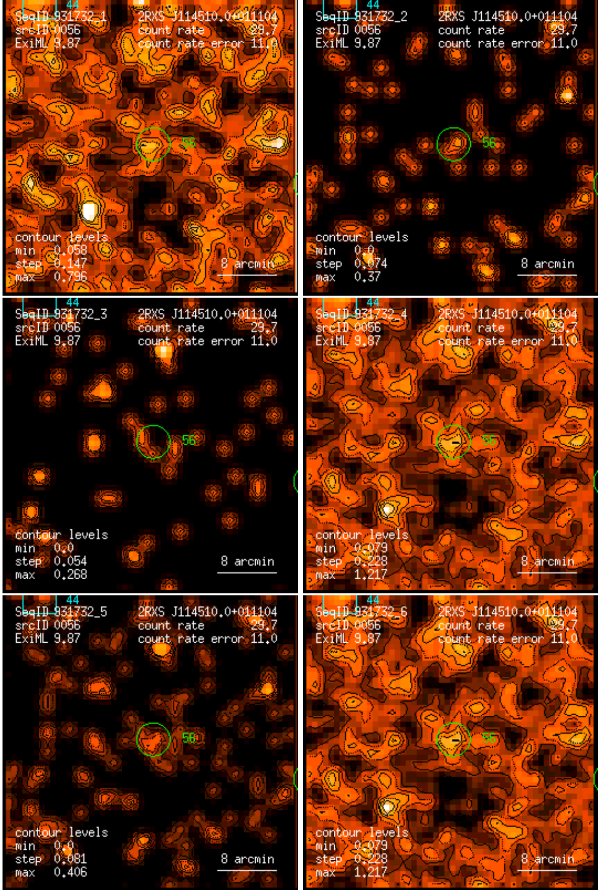
Figure 56: RASS 931732: detection 0056: band rate images, Gaussian filter: (1) PSPC channels 11 – 41, (2) 52 – 90, (3) 91 – 201, (4) 11 – 235, (5) 52 – 201, (6) 11 – 201. Broad band rates in counts/ks. Band rate contour levels in counts/ks/arcmin 2 .
