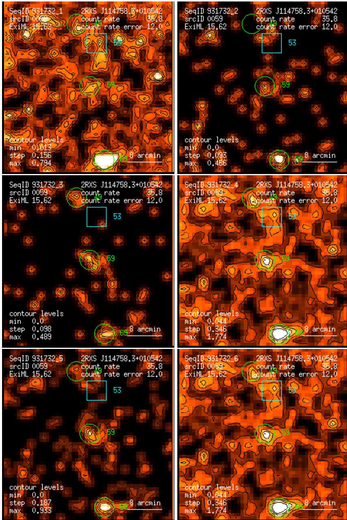
Figure 59: RASS 931732: detection 0059: band rate images, Gaussian filter: (1) PSPC channels 11 – 41, (2) 52 – 90, (3) 91 – 201, (4) 11 – 235, (5) 52 – 201, (6) 11 – 201. Broad band rates in counts/ks. Band rate contour levels in counts/ks/arcmin 2 .
