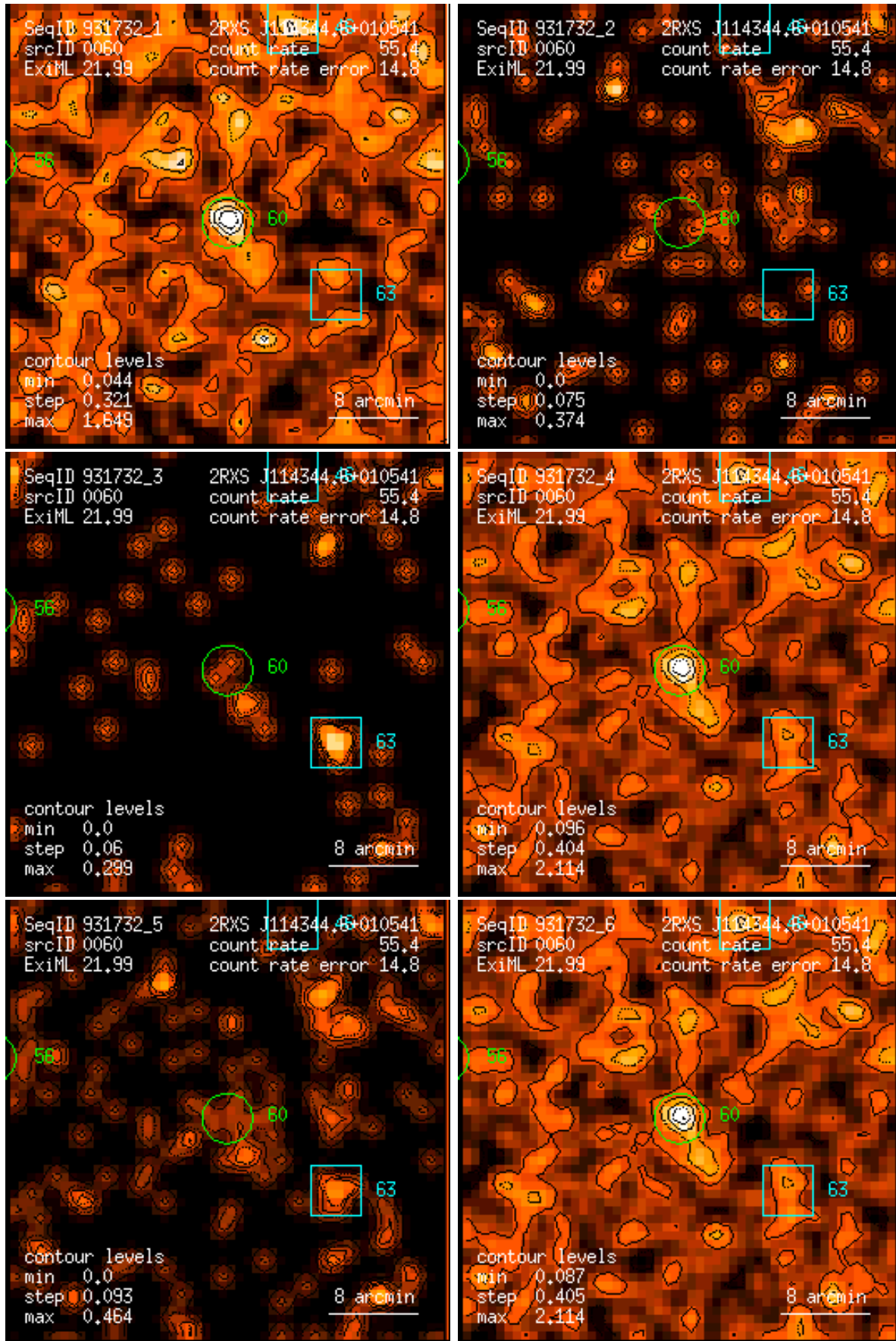
Figure 60: RASS 931732: detection 0060: band rate images, Gaussian filter: (1) PSPC channels 11 – 41, (2) 52 – 90, (3) 91 – 201, (4) 11 – 235, (5) 52 – 201, (6) 11 – 201. Broad band rates in counts/ks. Band rate contour levels in counts/ks/arcmin 2 .
