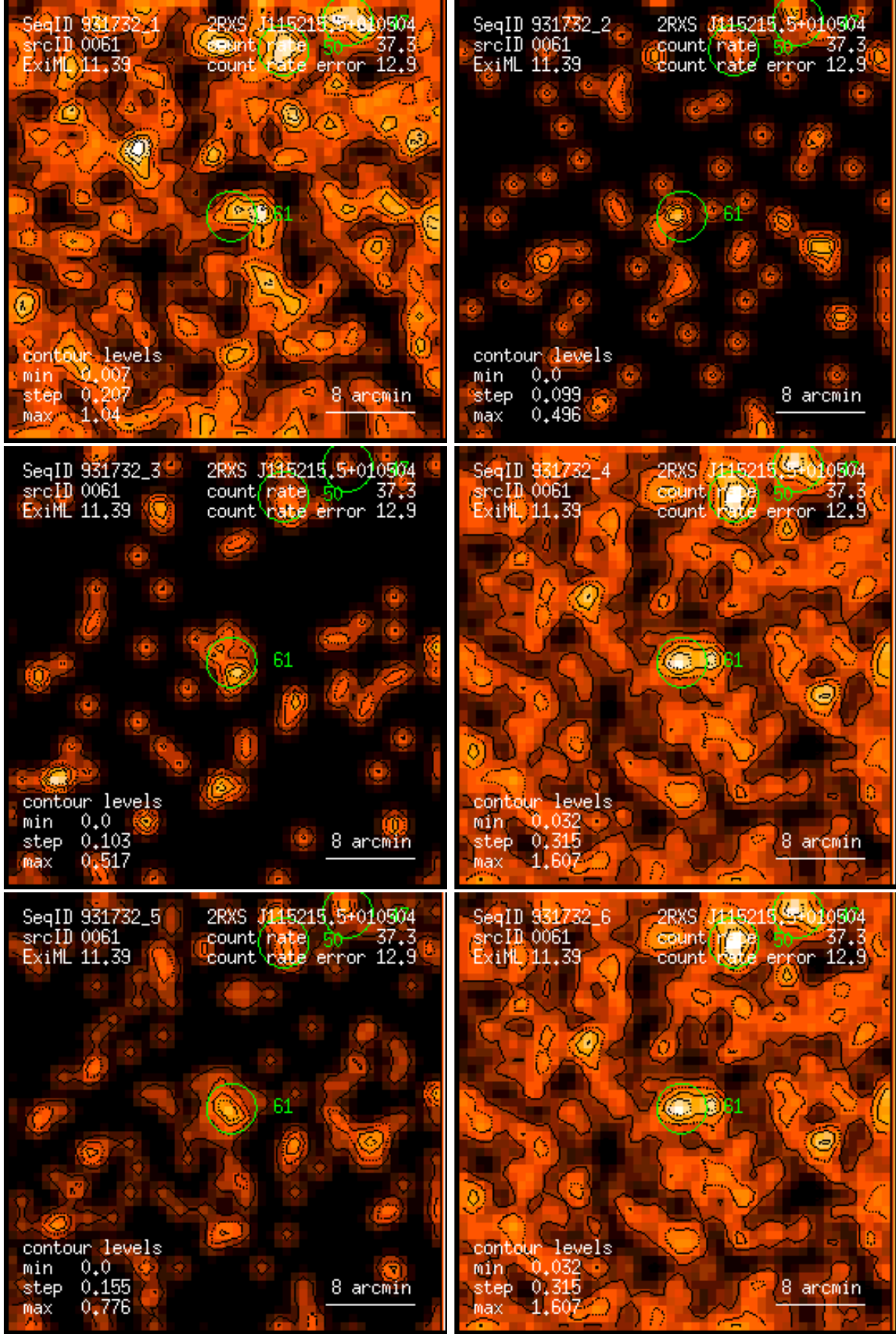
Figure 61: RASS 931732: detection 0061: band rate images, Gaussian filter: (1) PSPC channels 11 – 41, (2) 52 – 90, (3) 91 – 201, (4) 11 – 235, (5) 52 – 201, (6) 11 – 201. Broad band rates in counts/ks. Band rate contour levels in counts/ks/arcmin 2 .
