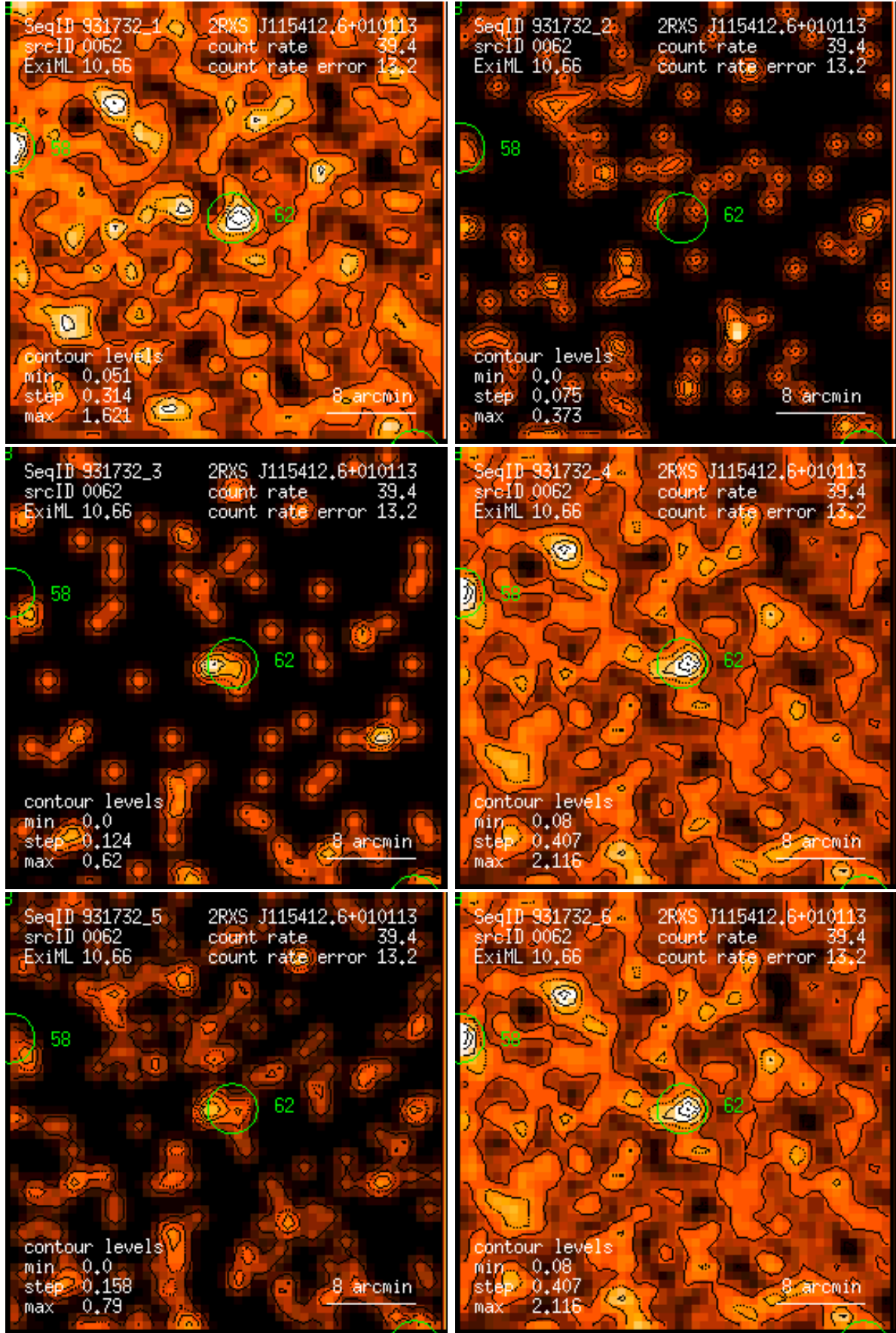
Figure 62: RASS 931732: detection 0062: band rate images, Gaussian filter: (1) PSPC channels 11 – 41, (2) 52 – 90, (3) 91 – 201, (4) 11 – 235, (5) 52 – 201, (6) 11 – 201. Broad band rates in counts/ks. Band rate contour levels in counts/ks/arcmin 2 .
