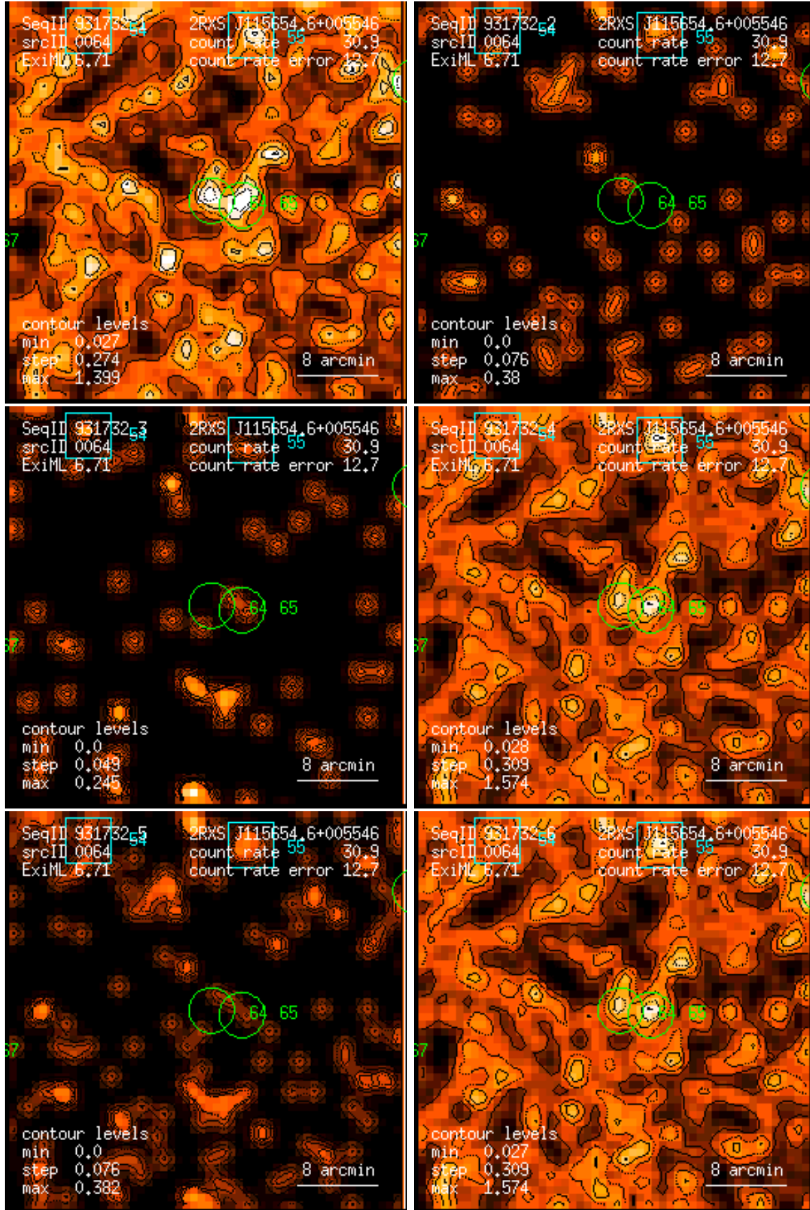
Figure 64: RASS 931732: detection 0064: band rate images, Gaussian filter: (1) PSPC channels 11 – 41, (2) 52 – 90, (3) 91 – 201, (4) 11 – 235, (5) 52 – 201, (6) 11 – 201. Broad band rates in counts/ks. Band rate contour levels in counts/ks/arcmin 2 .
