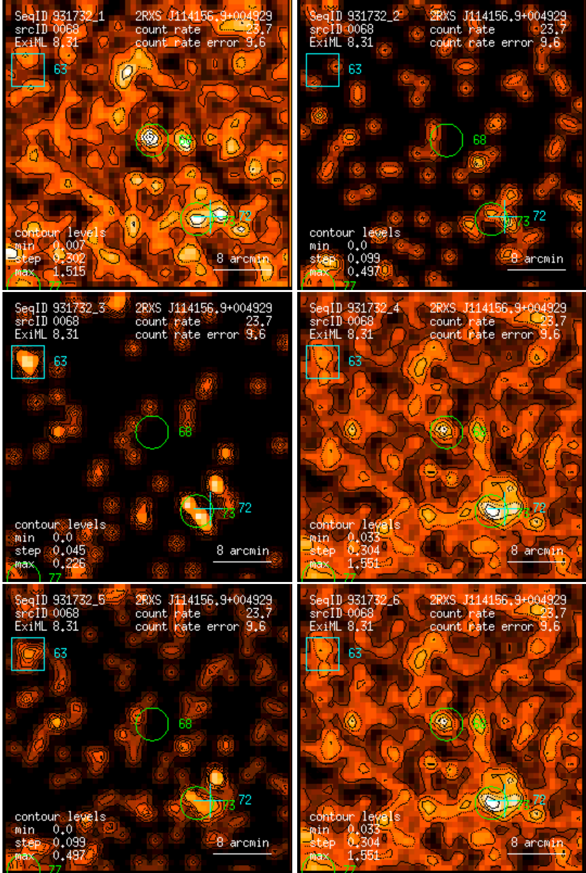
Figure 68: RASS 931732: detection 0068: band rate images, Gaussian filter: (1) PSPC channels 11 – 41, (2) 52 – 90, (3) 91 – 201, (4) 11 – 235, (5) 52 – 201, (6) 11 – 201. Broad band rates in counts/ks. Band rate contour levels in counts/ks/arcmin 2 .
