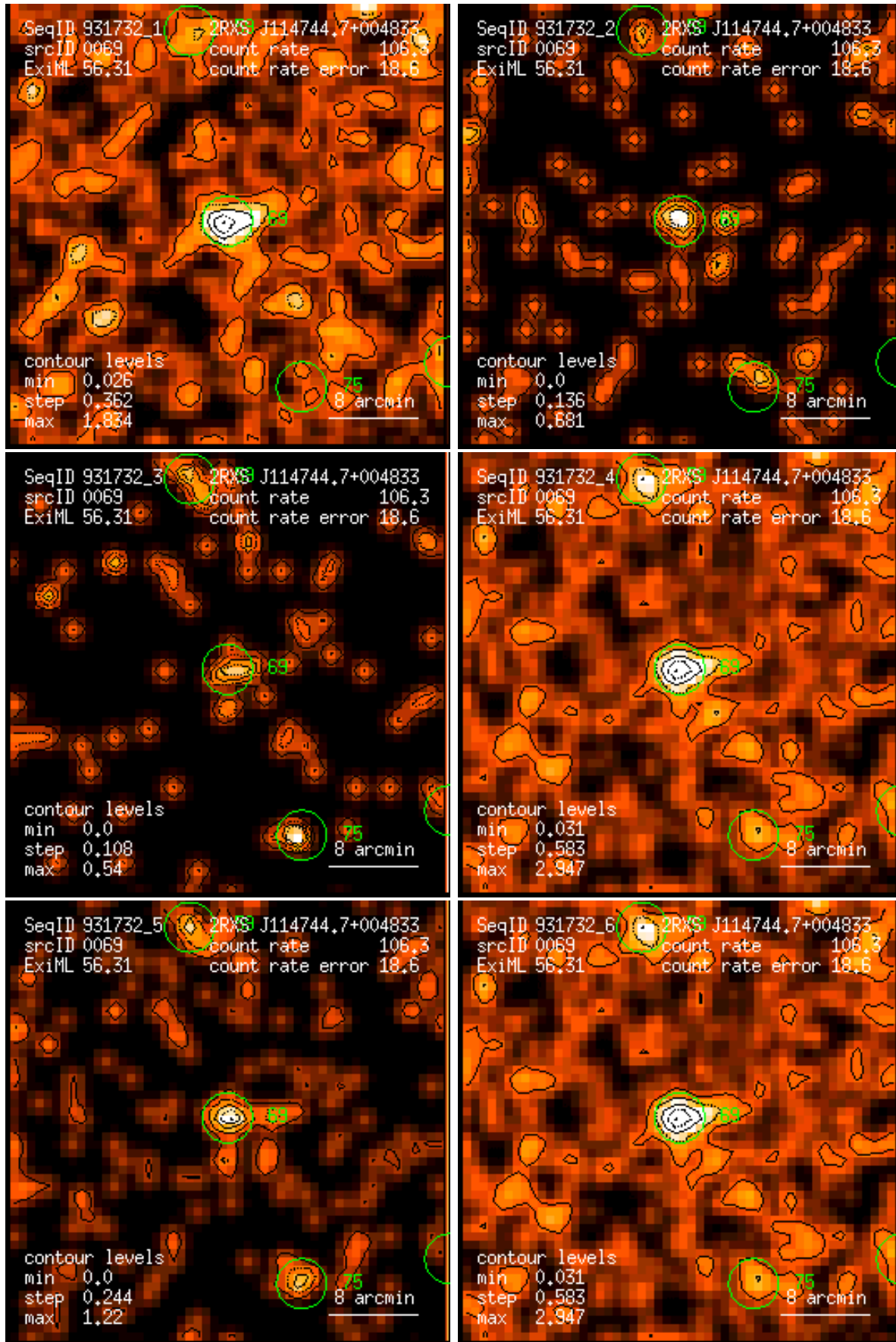
Figure 69: RASS 931732: detection 0069: band rate images, Gaussian filter: (1) PSPC channels 11 – 41, (2) 52 – 90, (3) 91 – 201, (4) 11 – 235, (5) 52 – 201, (6) 11 – 201. Broad band rates in counts/ks. Band rate contour levels in counts/ks/arcmin 2 .
