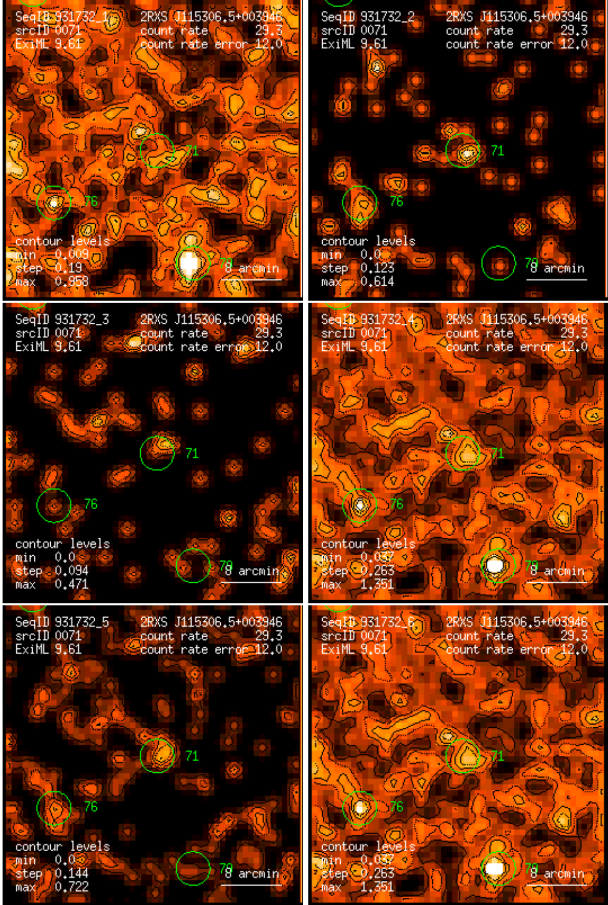
Figure 71: RASS 931732: detection 0071: band rate images, Gaussian filter: (1) PSPC channels 11 – 41, (2) 52 – 90, (3) 91 – 201, (4) 11 – 235, (5) 52 – 201, (6) 11 – 201. Broad band rates in counts/ks. Band rate contour levels in counts/ks/arcmin 2 .
