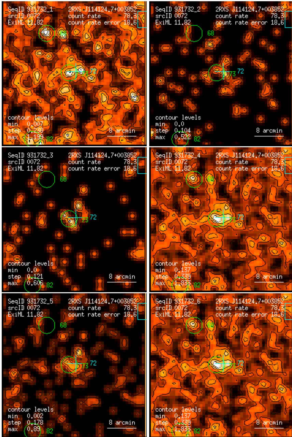
Figure 72: RASS 931732: detection 0072: band rate images, Gaussian filter: (1) PSPC channels 11 – 41, (2) 52 – 90, (3) 91 – 201, (4) 11 – 235, (5) 52 – 201, (6) 11 – 201. Broad band rates in counts/ks. Band rate contour levels in counts/ks/arcmin 2 .
