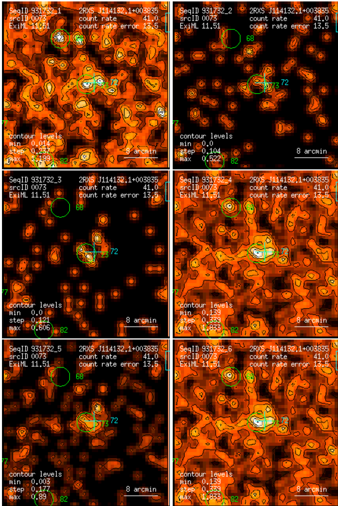
Figure 73: RASS 931732: detection 0073: band rate images, Gaussian filter: (1) PSPC channels 11 – 41, (2) 52 – 90, (3) 91 – 201, (4) 11 – 235, (5) 52 – 201, (6) 11 – 201. Broad band rates in counts/ks. Band rate contour levels in counts/ks/arcmin 2 .
