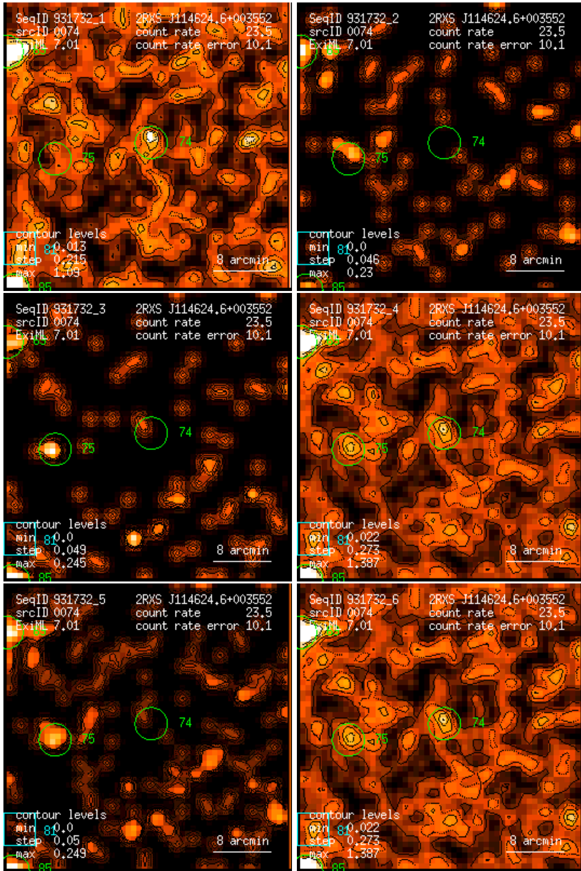
Figure 74: RASS 931732: detection 0074: band rate images, Gaussian filter: (1) PSPC channels 11 – 41, (2) 52 – 90, (3) 91 – 201, (4) 11 – 235, (5) 52 – 201, (6) 11 – 201. Broad band rates in counts/ks. Band rate contour levels in counts/ks/arcmin 2 .
