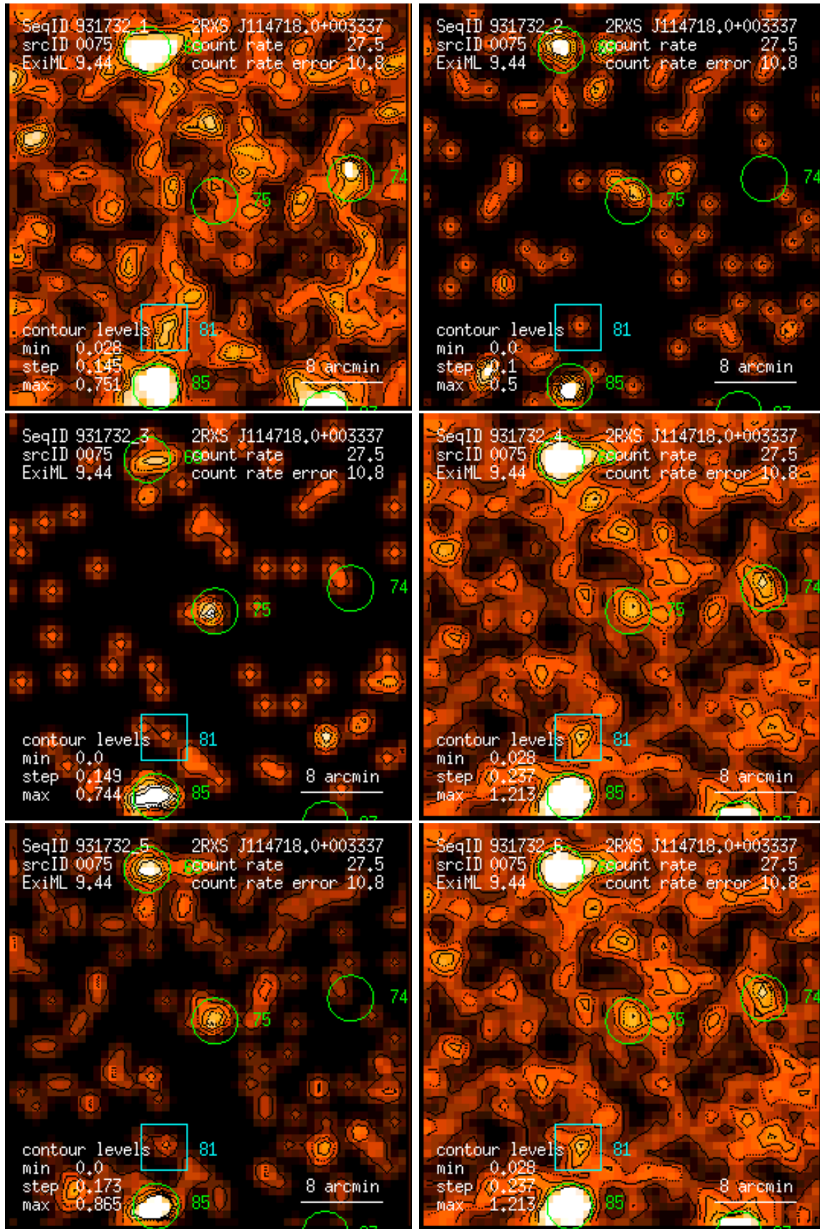
Figure 75: RASS 931732: detection 0075: band rate images, Gaussian filter: (1) PSPC channels 11 – 41, (2) 52 – 90, (3) 91 – 201, (4) 11 – 235, (5) 52 – 201, (6) 11 – 201. Broad band rates in counts/ks. Band rate contour levels in counts/ks/arcmin 2 .
