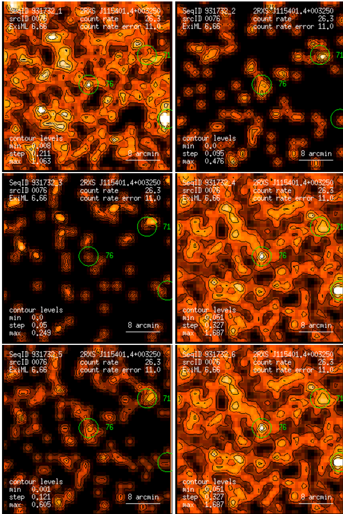
Figure 76: RASS 931732: detection 0076: band rate images, Gaussian filter: (1) PSPC channels 11 – 41, (2) 52 – 90, (3) 91 – 201, (4) 11 – 235, (5) 52 – 201, (6) 11 – 201. Broad band rates in counts/ks. Band rate contour levels in counts/ks/arcmin 2 .
