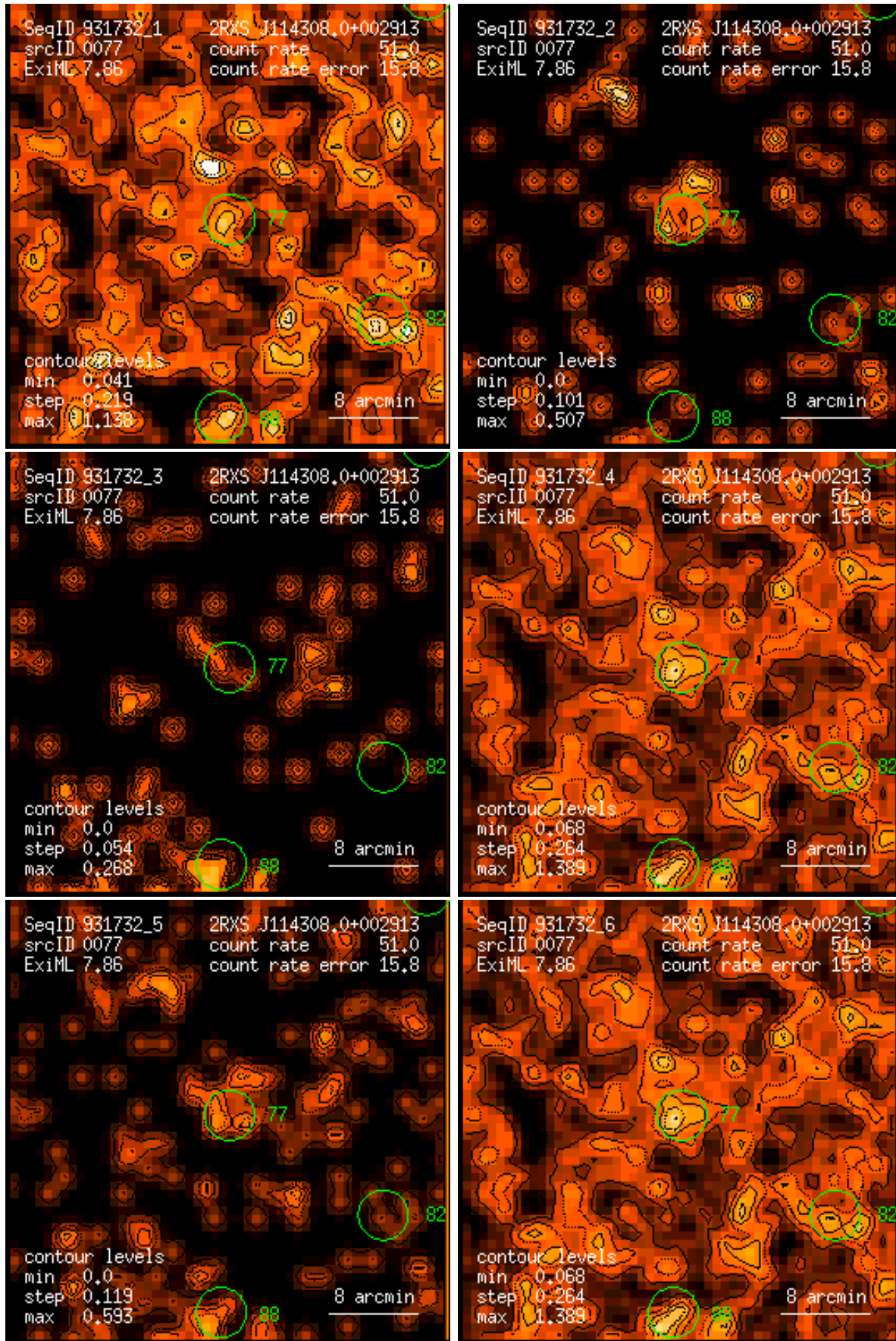
Figure 77: RASS 931732: detection 0077: band rate images, Gaussian filter: (1) PSPC channels 11 – 41, (2) 52 – 90, (3) 91 – 201, (4) 11 – 235, (5) 52 – 201, (6) 11 – 201. Broad band rates in counts/ks. Band rate contour levels in counts/ks/arcmin 2 .
