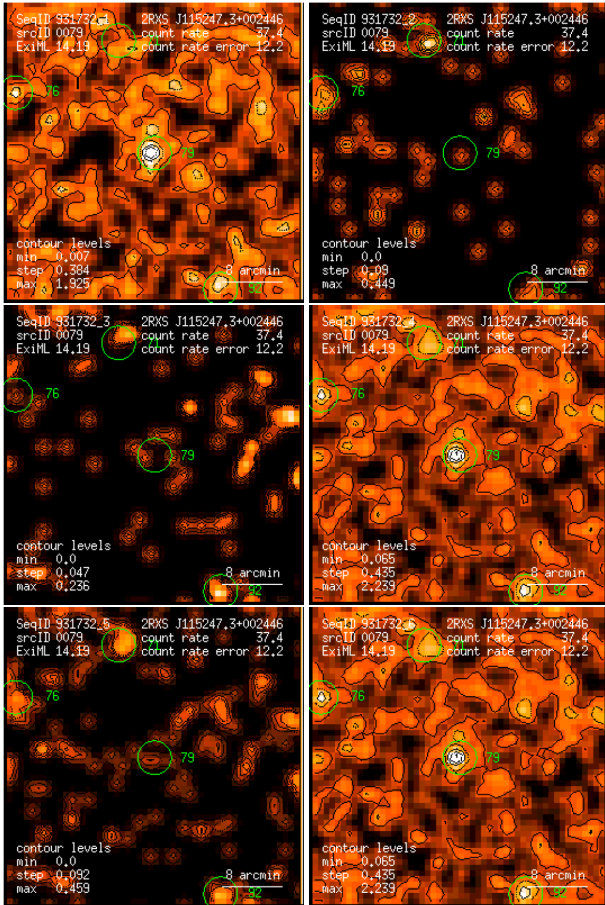
Figure 79: RASS 931732: detection 0079: band rate images, Gaussian filter: (1) PSPC channels 11 – 41, (2) 52 – 90, (3) 91 – 201, (4) 11 – 235, (5) 52 – 201, (6) 11 – 201. Broad band rates in counts/ks. Band rate contour levels in counts/ks/arcmin 2 .
