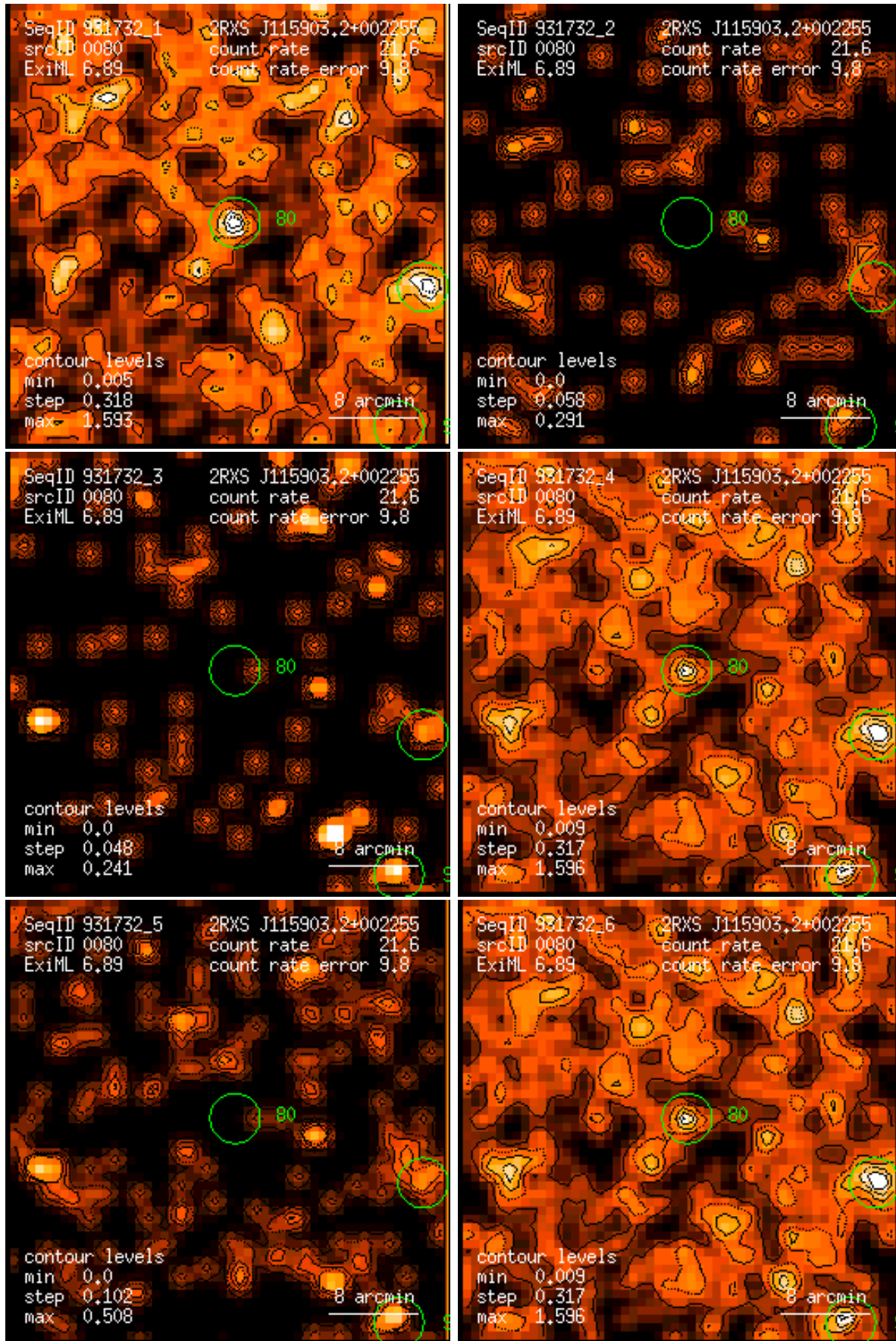
Figure 80: RASS 931732: detection 0080: band rate images, Gaussian filter: (1) PSPC channels 11 – 41, (2) 52 – 90, (3) 91 – 201, (4) 11 – 235, (5) 52 – 201, (6) 11 – 201. Broad band rates in counts/ks. Band rate contour levels in counts/ks/arcmin 2 .
