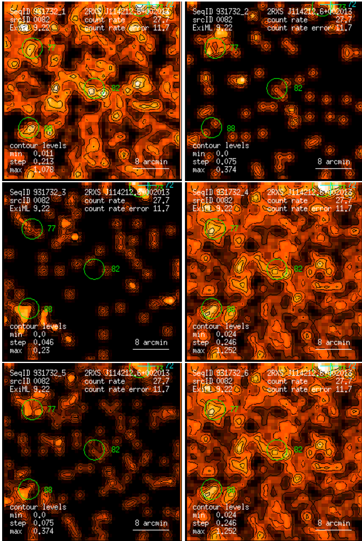
Figure 82: RASS 931732: detection 0082: band rate images, Gaussian filter: (1) PSPC channels 11 – 41, (2) 52 – 90, (3) 91 – 201, (4) 11 – 235, (5) 52 – 201, (6) 11 – 201. Broad band rates in counts/ks. Band rate contour levels in counts/ks/arcmin 2 .
