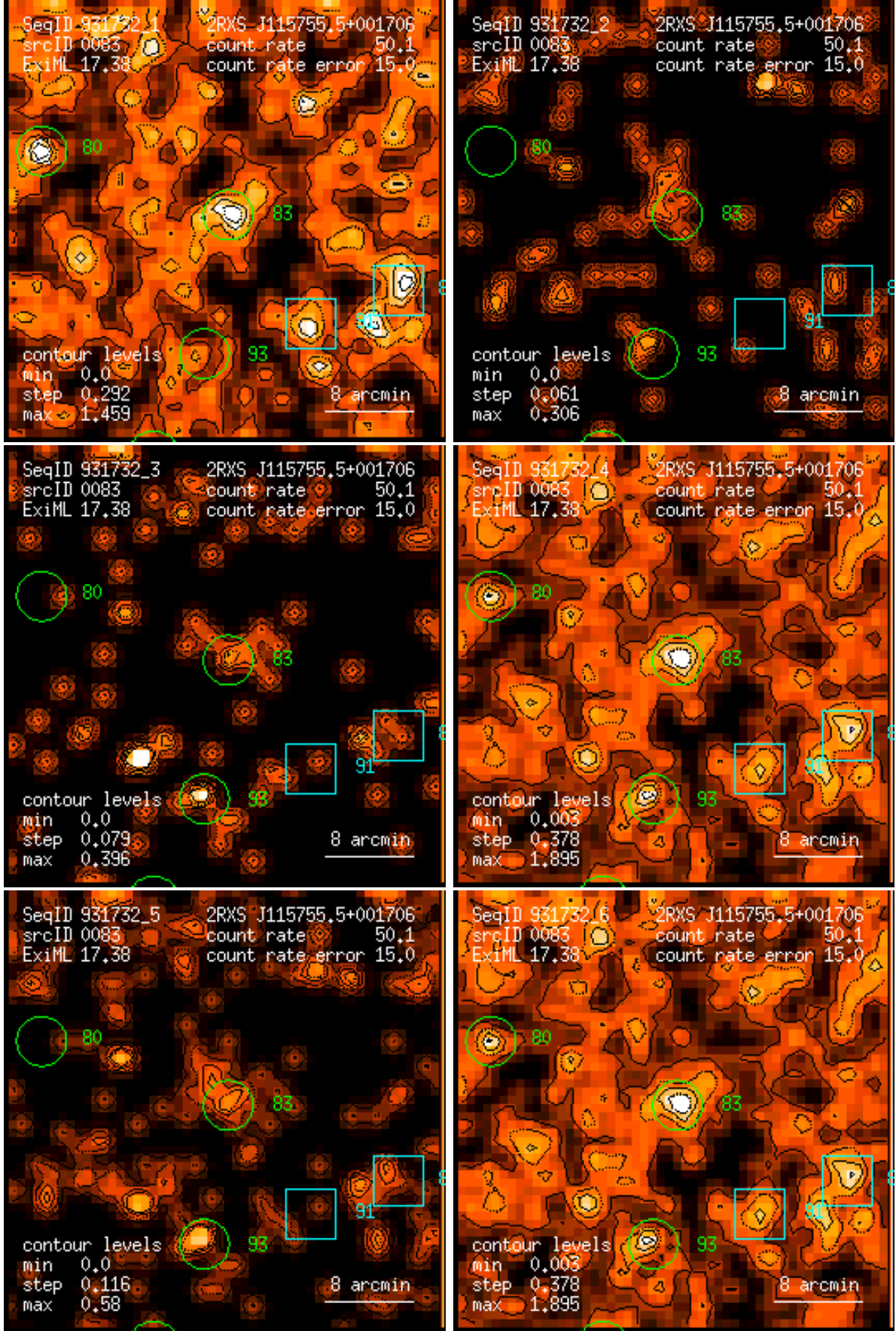
Figure 83: RASS 931732: detection 0083: band rate images, Gaussian filter: (1) PSPC channels 11 – 41, (2) 52 – 90, (3) 91 – 201, (4) 11 – 235, (5) 52 – 201, (6) 11 – 201. Broad band rates in counts/ks. Band rate contour levels in counts/ks/arcmin 2 .
