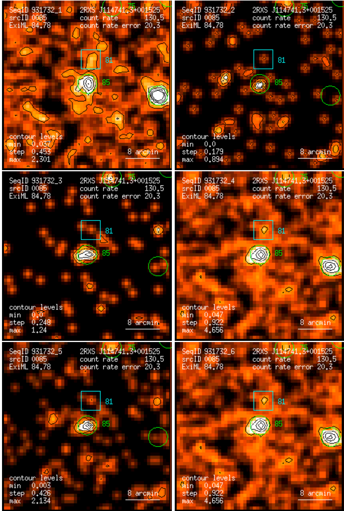
Figure 85: RASS 931732: detection 0085: band rate images, Gaussian filter: (1) PSPC channels 11 – 41, (2) 52 – 90, (3) 91 – 201, (4) 11 – 235, (5) 52 – 201, (6) 11 – 201. Broad band rates in counts/ks. Band rate contour levels in counts/ks/arcmin 2 .
