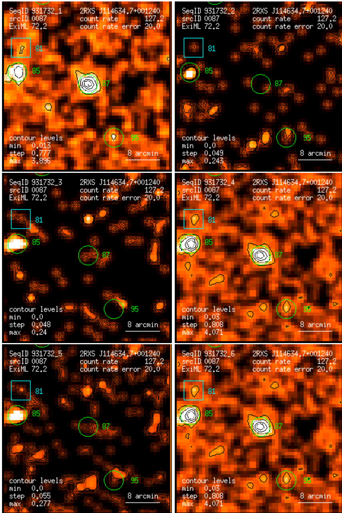
Figure 87: RASS 931732: detection 0087: band rate images, Gaussian filter: (1) PSPC channels 11 – 41, (2) 52 – 90, (3) 91 – 201, (4) 11 – 235, (5) 52 – 201, (6) 11 – 201. Broad band rates in counts/ks. Band rate contour levels in counts/ks/arcmin 2 .
