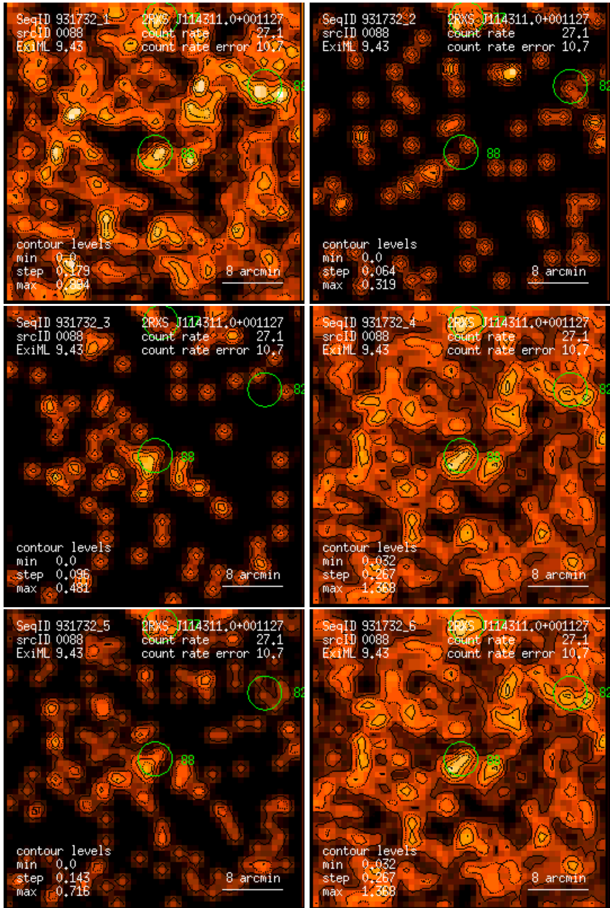
Figure 88: RASS 931732: detection 0088: band rate images, Gaussian filter: (1) PSPC channels 11 – 41, (2) 52 – 90, (3) 91 – 201, (4) 11 – 235, (5) 52 – 201, (6) 11 – 201. Broad band rates in counts/ks. Band rate contour levels in counts/ks/arcmin 2 .
