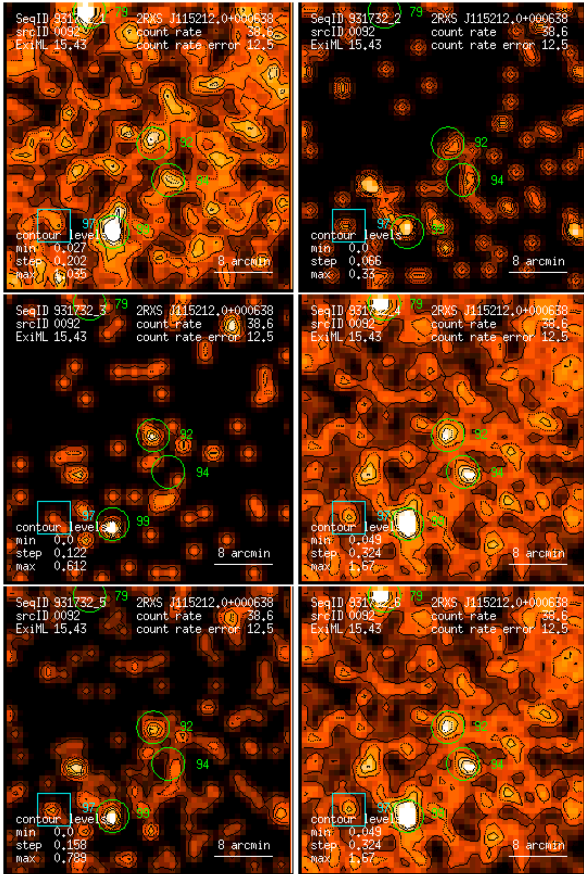
Figure 92: RASS 931732: detection 0092: band rate images, Gaussian filter: (1) PSPC channels 11 – 41, (2) 52 – 90, (3) 91 – 201, (4) 11 – 235, (5) 52 – 201, (6) 11 – 201. Broad band rates in counts/ks. Band rate contour levels in counts/ks/arcmin 2 .
