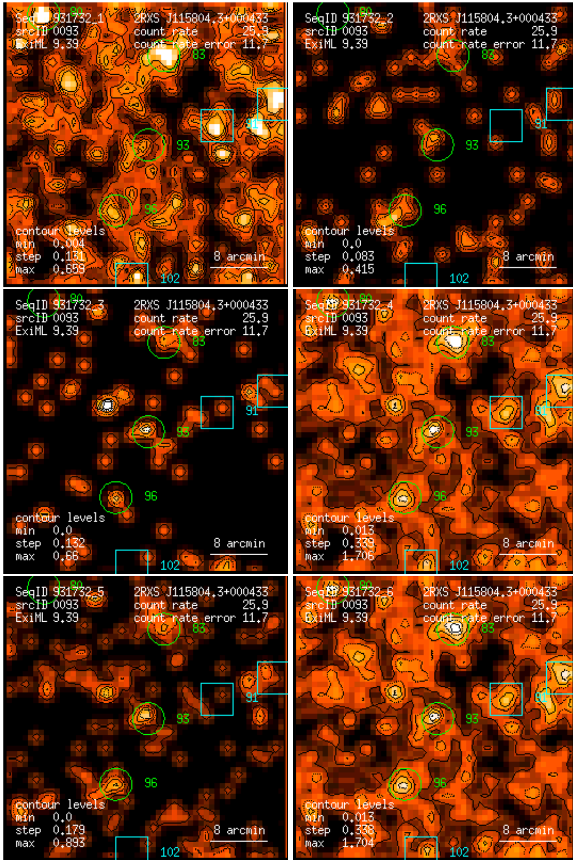
Figure 93: RASS 931732: detection 0093: band rate images, Gaussian filter: (1) PSPC channels 11 – 41, (2) 52 – 90, (3) 91 – 201, (4) 11 – 235, (5) 52 – 201, (6) 11 – 201. Broad band rates in counts/ks. Band rate contour levels in counts/ks/arcmin 2 .
