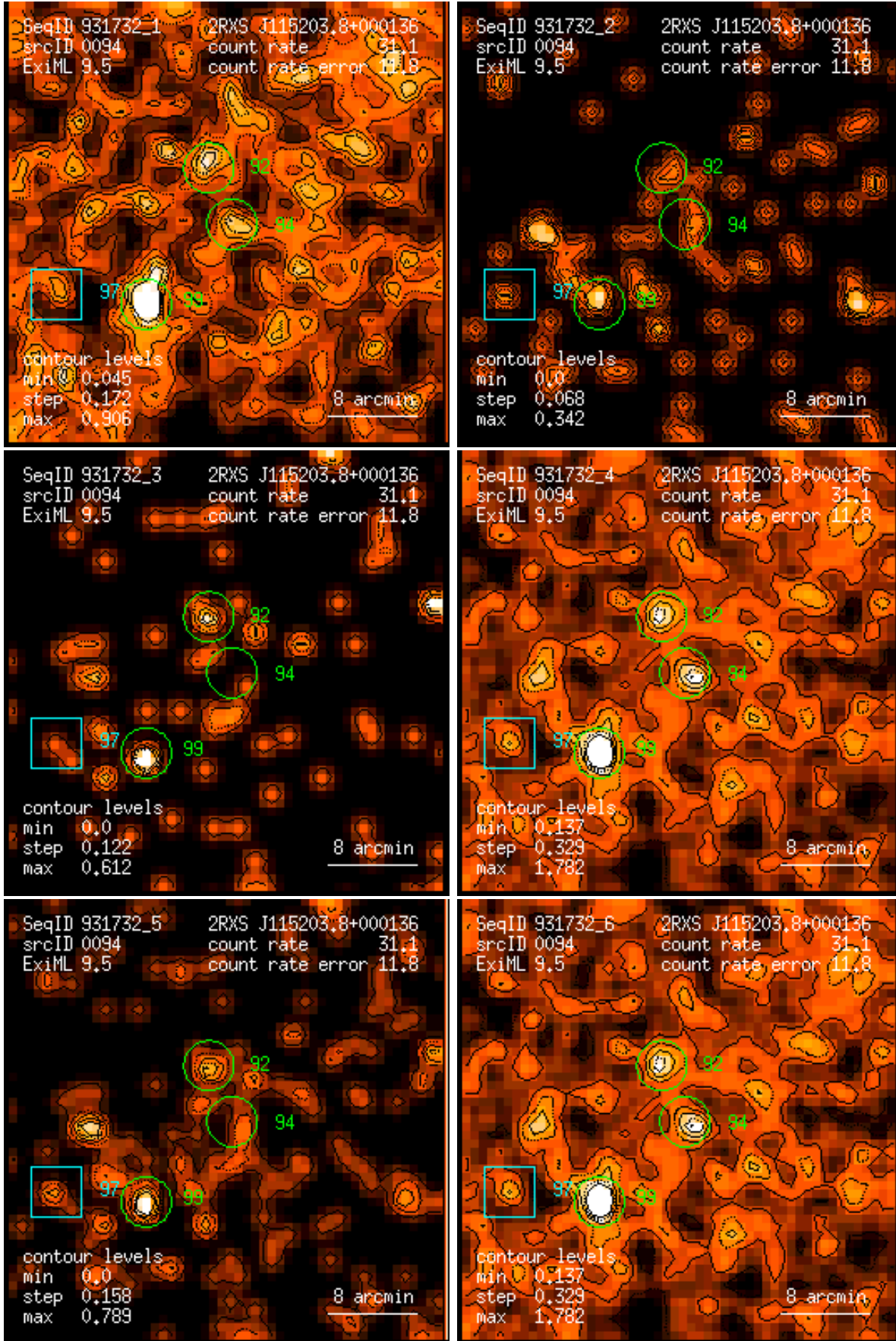
Figure 94: RASS 931732: detection 0094: band rate images, Gaussian filter: (1) PSPC channels 11 – 41, (2) 52 – 90, (3) 91 – 201, (4) 11 – 235, (5) 52 – 201, (6) 11 – 201. Broad band rates in counts/ks. Band rate contour levels in counts/ks/arcmin 2 .
