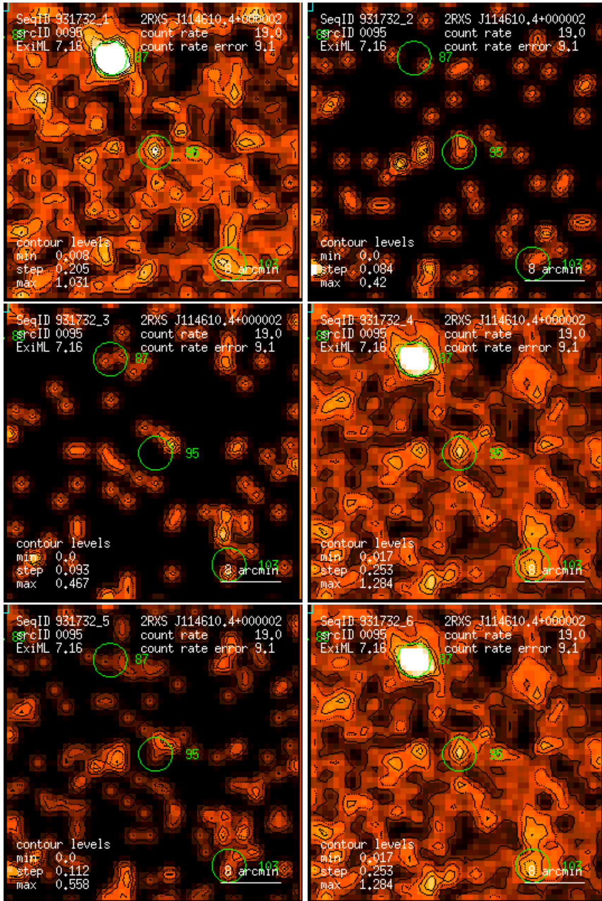
Figure 95: RASS 931732: detection 0095: band rate images, Gaussian filter: (1) PSPC channels 11 – 41, (2) 52 – 90, (3) 91 – 201, (4) 11 – 235, (5) 52 – 201, (6) 11 – 201. Broad band rates in counts/ks. Band rate contour levels in counts/ks/arcmin 2 .
