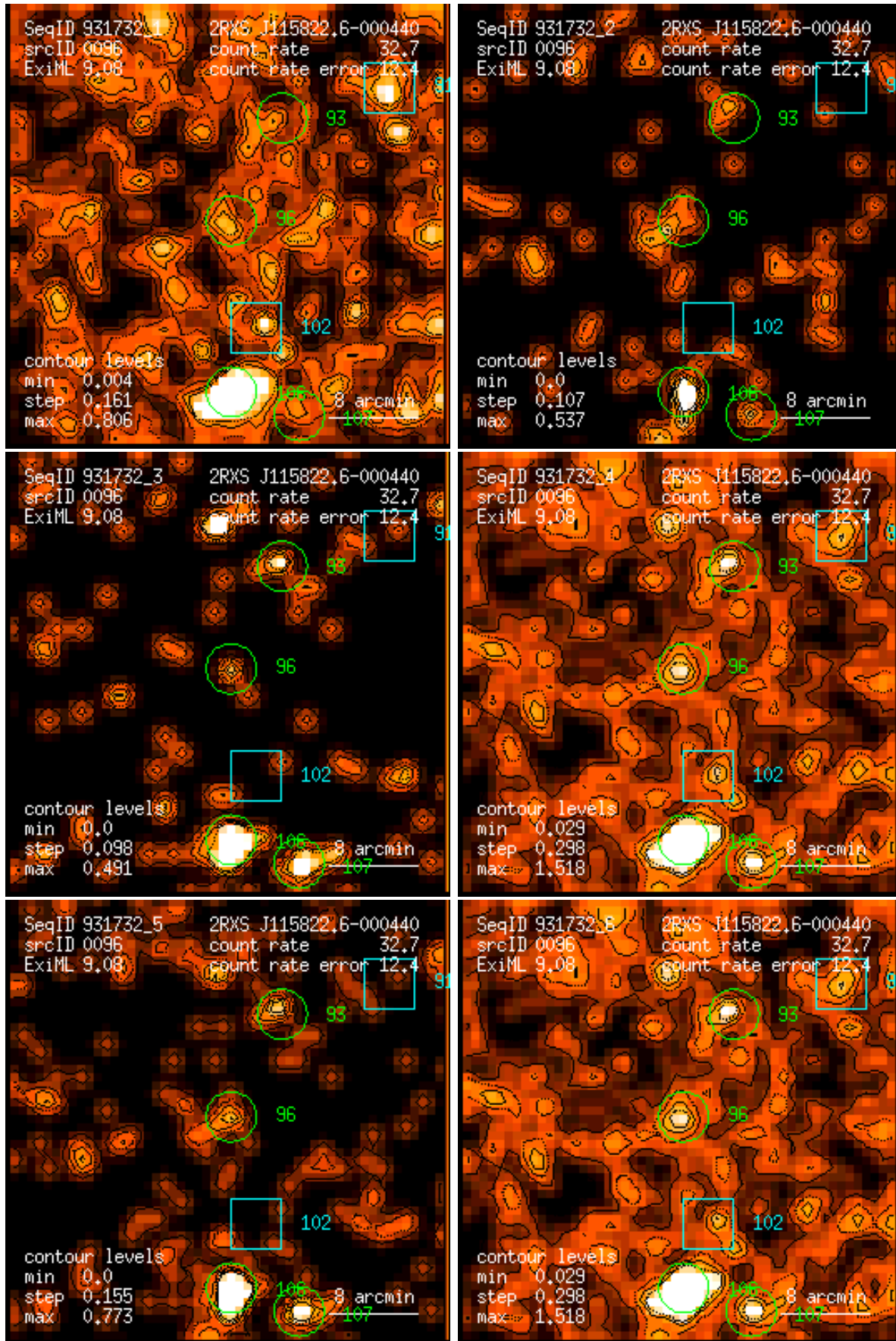
Figure 96: RASS 931732: detection 0096: band rate images, Gaussian filter: (1) PSPC channels 11 – 41, (2) 52 – 90, (3) 91 – 201, (4) 11 – 235, (5) 52 – 201, (6) 11 – 201. Broad band rates in counts/ks. Band rate contour levels in counts/ks/arcmin 2 .
