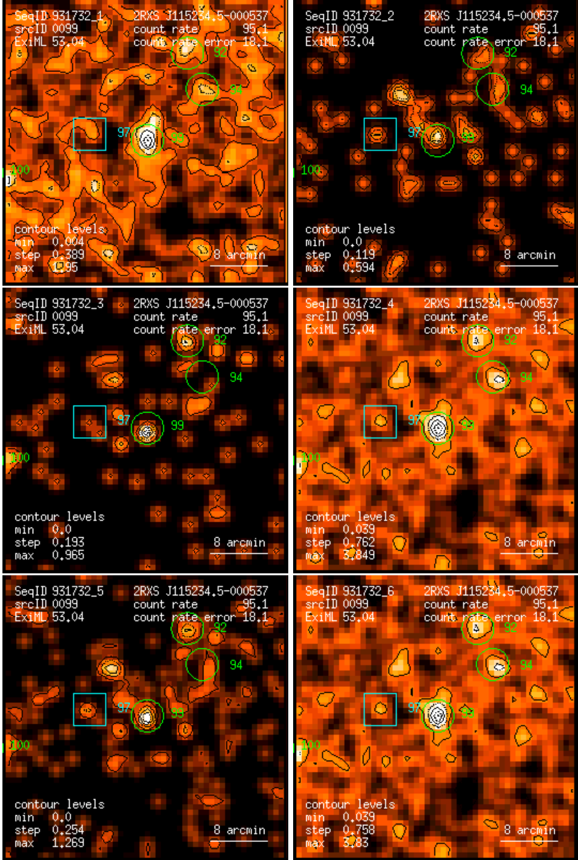
Figure 99: RASS 931732: detection 0099: band rate images, Gaussian filter: (1) PSPC channels 11 – 41, (2) 52 – 90, (3) 91 – 201, (4) 11 – 235, (5) 52 – 201, (6) 11 – 201. Broad band rates in counts/ks. Band rate contour levels in counts/ks/arcmin 2 .
