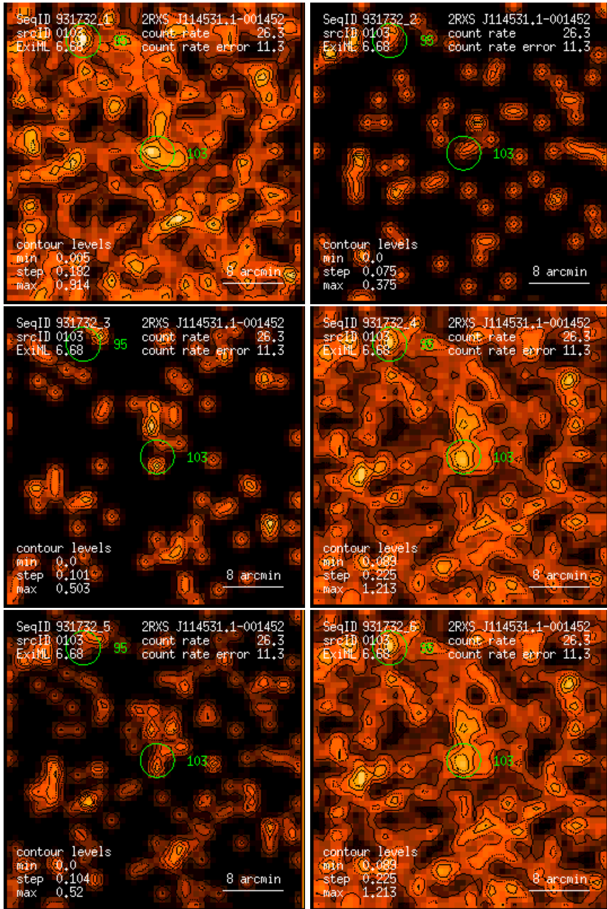
Figure 103: RASS 931732: detection 0103: band rate images, Gaussian filter: (1) PSPC channels 11 – 41, (2) 52 – 90, (3) 91 – 201, (4) 11 – 235, (5) 52 – 201, (6) 11 – 201. Broad band rates in counts/ks. Band rate contour levels in counts/ks/arcmin 2 .
